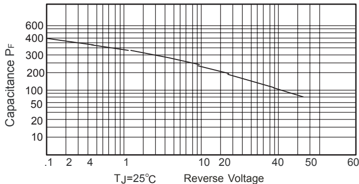
FIG.2-JUNCTION CAPACITANCE
