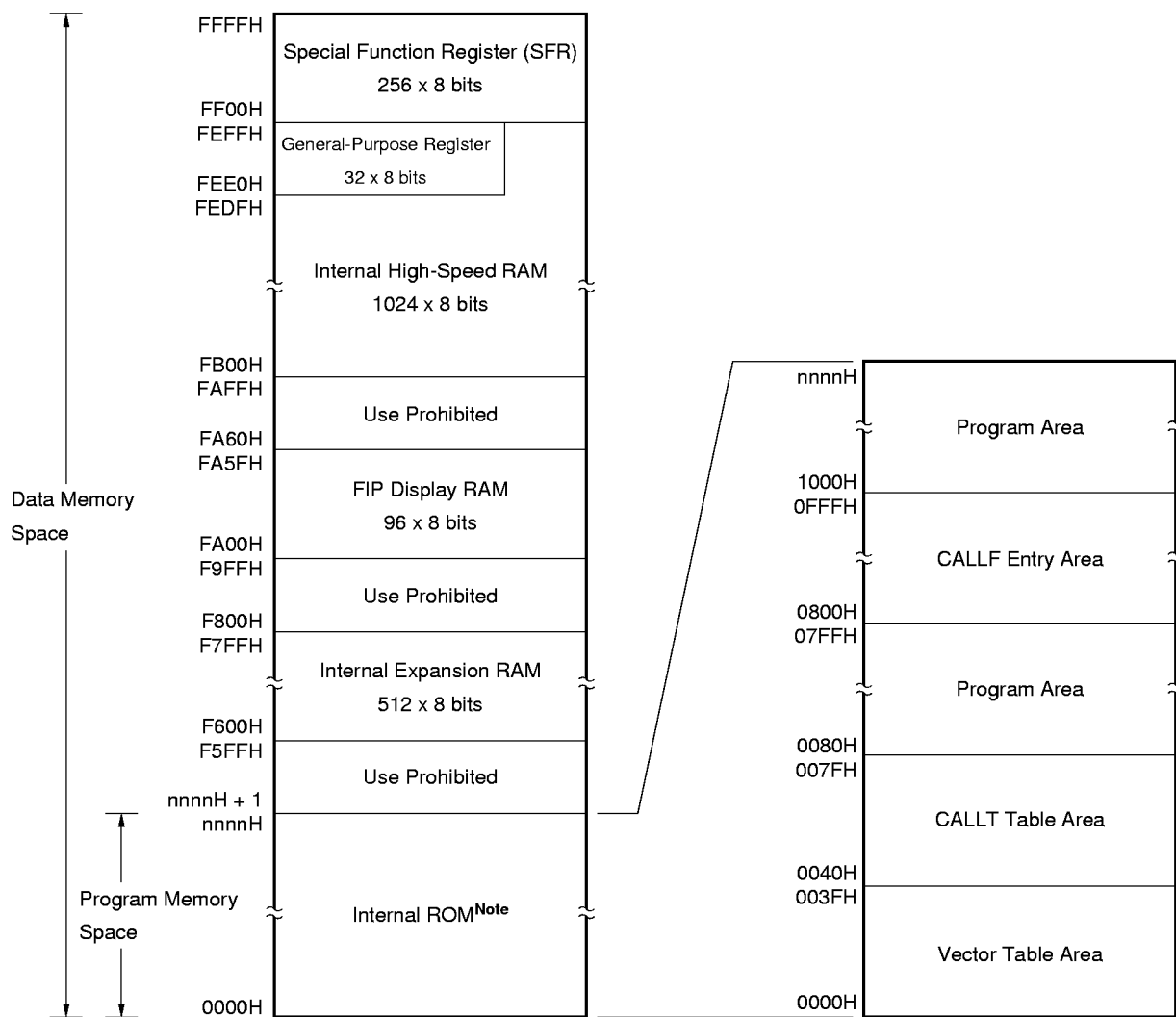
Figure 4-1. Memory Map
