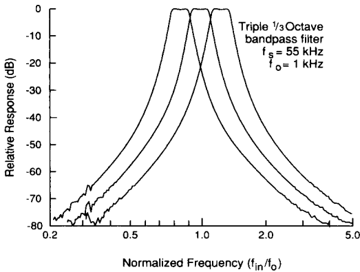
Figure 4. Frequency Response
