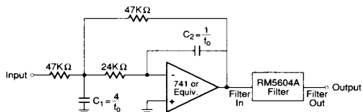
Figure 2. Test Circuit
