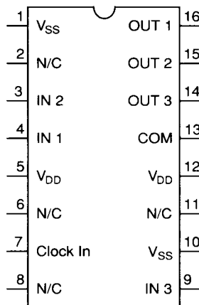
Figure 1. Pinout Configuration
