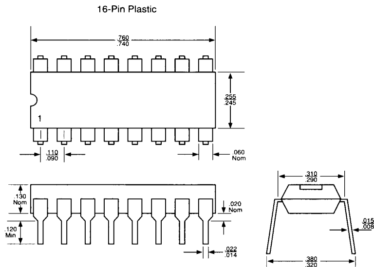
Figure 5. Package Dimensions
