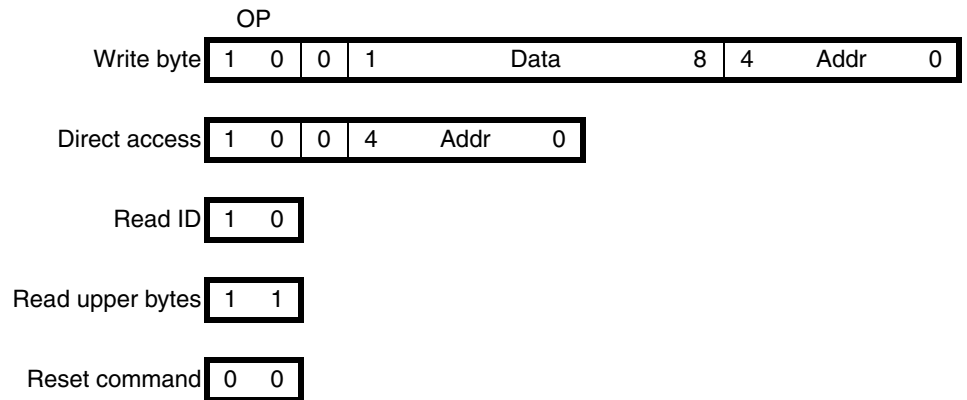
Figure 5-4. ATA5575M2 Command Formats
