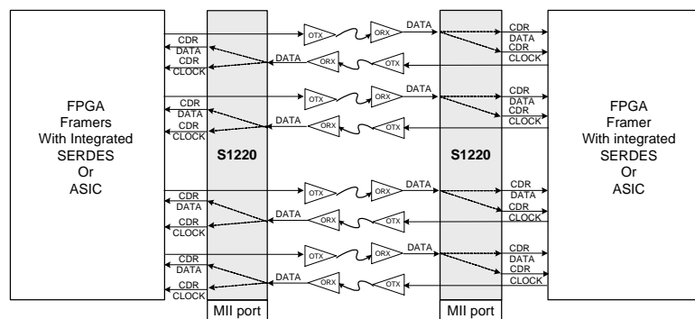
System Block Diagram with the S1220
