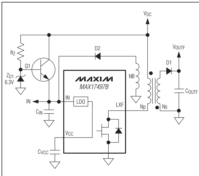
Figure 7. MAX17497B Typical Startup Circuit with Bias Winding to Turn Off Q1 and Reduce Power Dissipation
