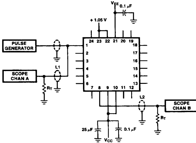
FIGURE 1. AC Test Circuit
