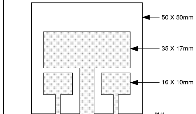
FIGURE 2. SUBSTRATE LAYOUT FOR SOT-223
