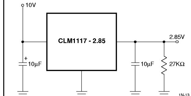
FIGURE 1. CIRCUIT LAYOUT, THERMAL EXPERIMENTS
