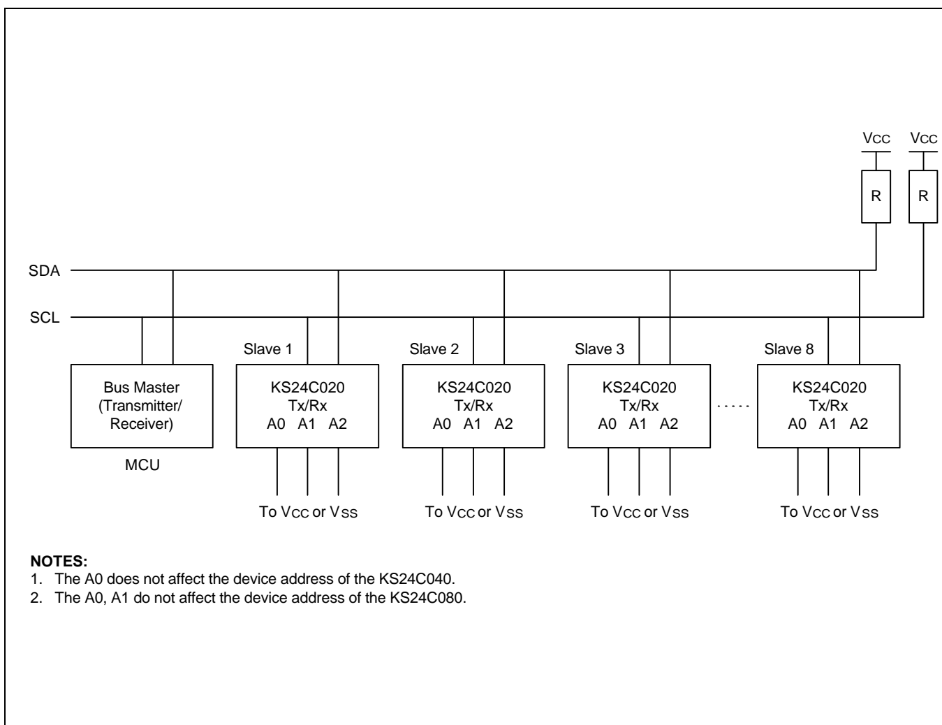
Figure 4-6. Typical Configuration (16 Kbits of Memory on the I 2 C-Bus)
