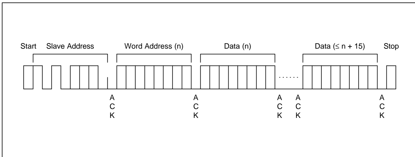
Figure 4-10. Page Write Operation
