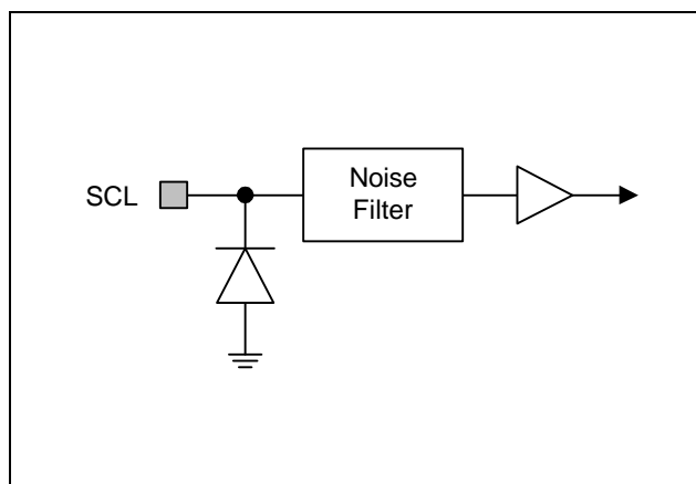
Figure 4-4. Pin Circuit Type 2
