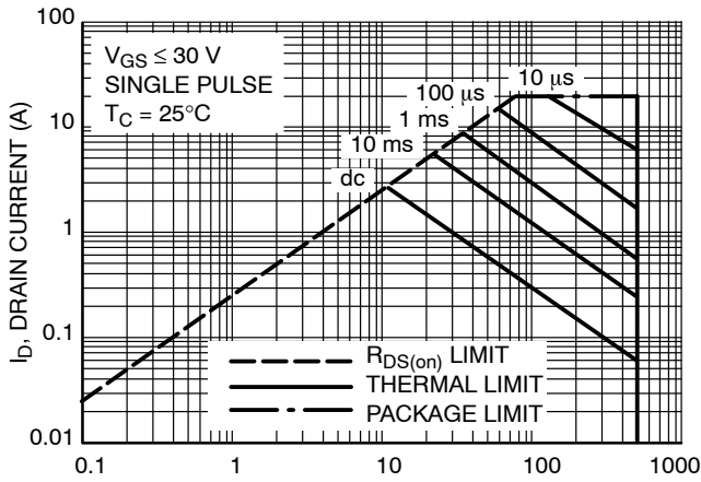
V_{DS} , DRAIN-TO-SOURCE VOLTAGE (V) Figure 12. Maximum Rated Forward Biased Safe Operating Area NDF05N50Z
