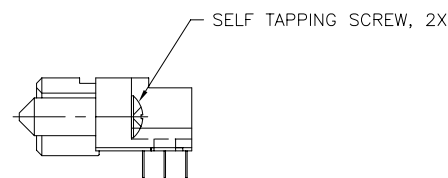
SECTION U-U
