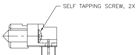
SECTION U-U
