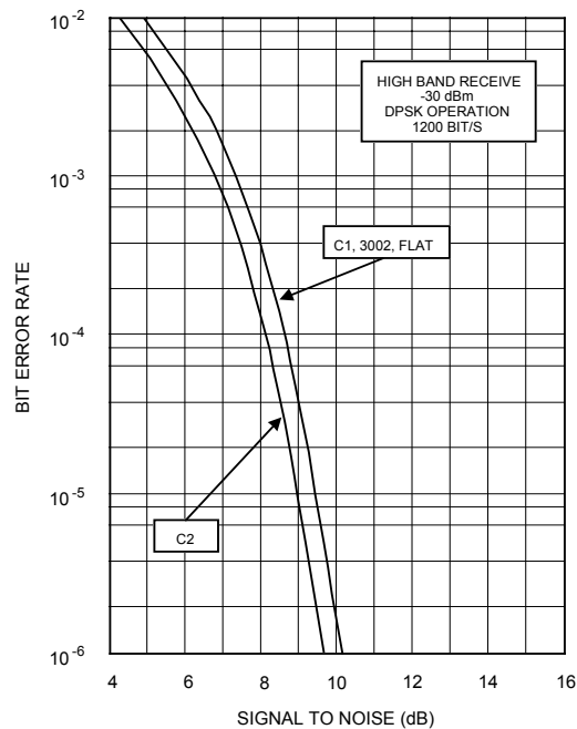
73K224BL BER vs S/N-DPSK HIGH BAND
