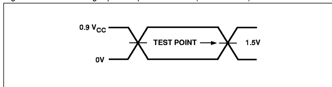
Figure 41B. AC Testing Input/Output Waveform (3 V Versions)
