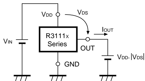
Detector Threshold Test Circuit
