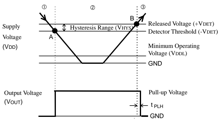
Figure 4. Operation Diagram
