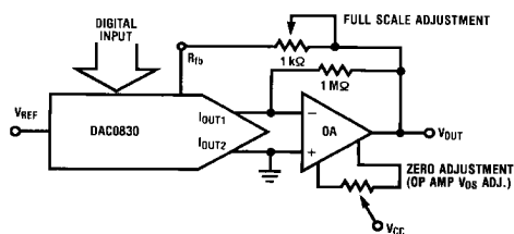
FIGURE 10. Adding Full-Scale Adjustment
