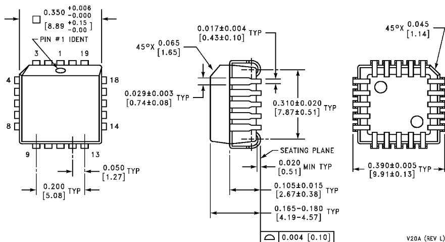
Molded Chip Carrier (V) Order Number DAC0830LCV or DAC0832LCV NS Package Number V20A
