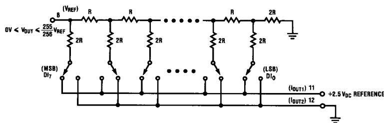
FIGURE 11. Voltage Mode Switching
