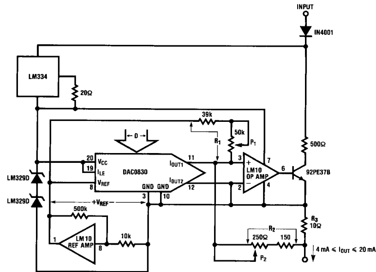
Two Terminal Floating 4 to 20 mA Current Loop Controller
