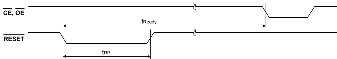
Figure 10. Reset Timings
