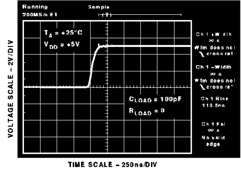
Figure 12. TMP04 Output Rise Time at +25°C
