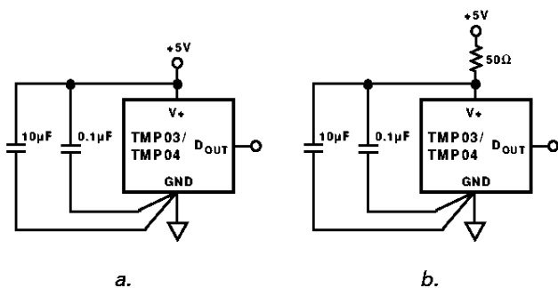
Figure 28. Recommended Supply Bypassing for the TMP03/TMP04
