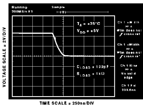
Figure 5. TMP03 Output Fall Time at +25°C
