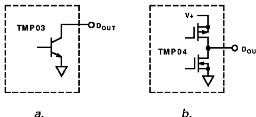
Figure 29. TMP03/TMP04 Digital Output Structure
