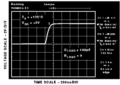
Figure 13. TMP04 Output Rise Time at +125°C
