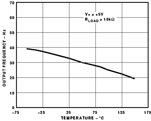
Figure 3. Output Frequency vs. Temperature
