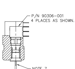
SECTION P-P
