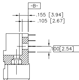
SECTION U-U
