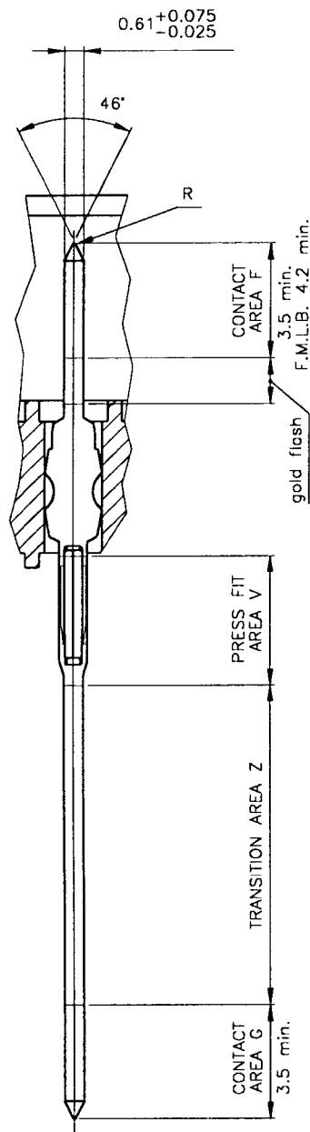
DETAIL P SCALE 10:1
