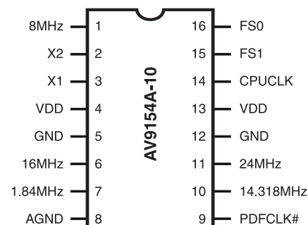
16-Pin PDIP or SOIC AV9154A-10
