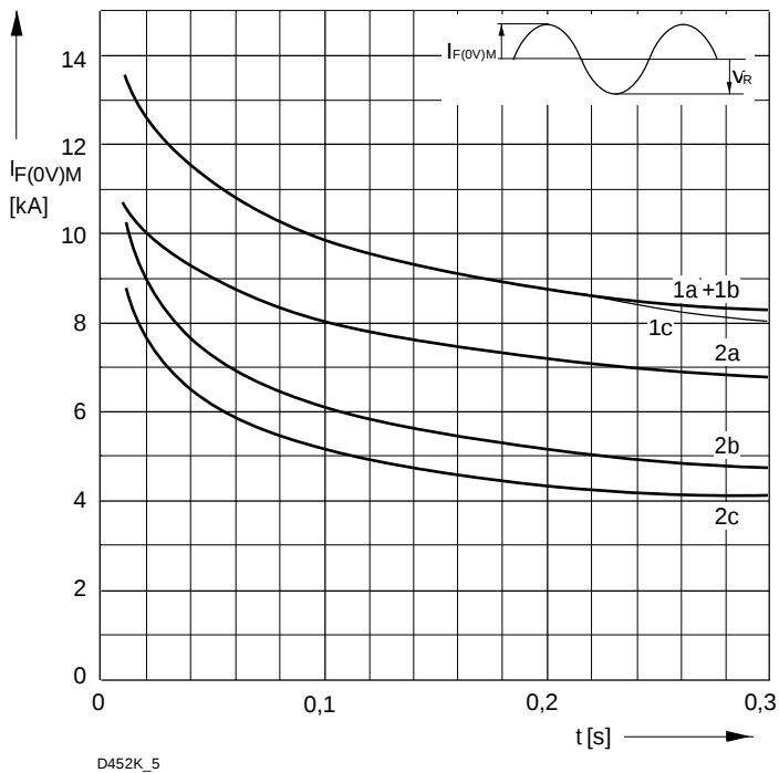
Bild / Fig. 3 Grenzstrom / Maximum overload forward current I_{F(0V)M} = f(t) 1 - I_{FAV(vor)} = 0\text{ A} ; t_{vj} = t_c = 25\text{ °C} 2 - I_{FAV(vor)} = 450\text{ A} ; t_c = 130\text{ °C} ; t_{vj} = 180\text{ °C} a - V_R \leq 50\text{ V} b - V_R = 0,5\text{ V}_{RRM} c - V_R = 0,8\text{ V}_{RRM}
