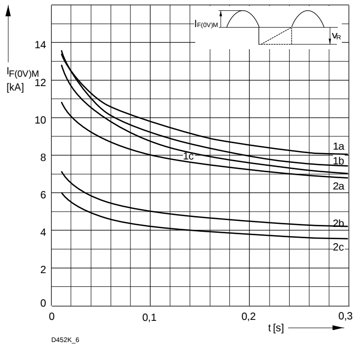
Bild / Fig. 4 Grenzstrom / Maximum overload forward current I_{F(0V)M} = f(t) 1 - I_{FAV(vor)} = 0\text{ A} ; t_{vj} = t_c = 25\text{ °C} 2 - I_{FAV(vor)} = 450\text{ A} ; t_c = 130\text{ °C} ; t_{vj} = 180\text{ °C} a - V_R \leq 50\text{ V} b - V_R = 0,5\text{ V}_{RRM} c - V_R = 0,8\text{ V}_{RRM}
