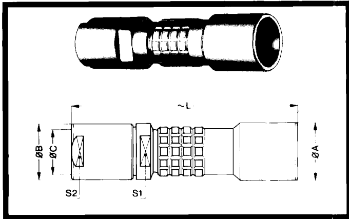
PCA Straight receptacle with oversized collet
