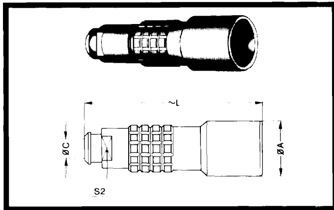
PCA Free receptacle with cable collet and backnut to accommodate a strain relief
