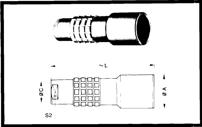
PCA Straight receptacle with cable collet
