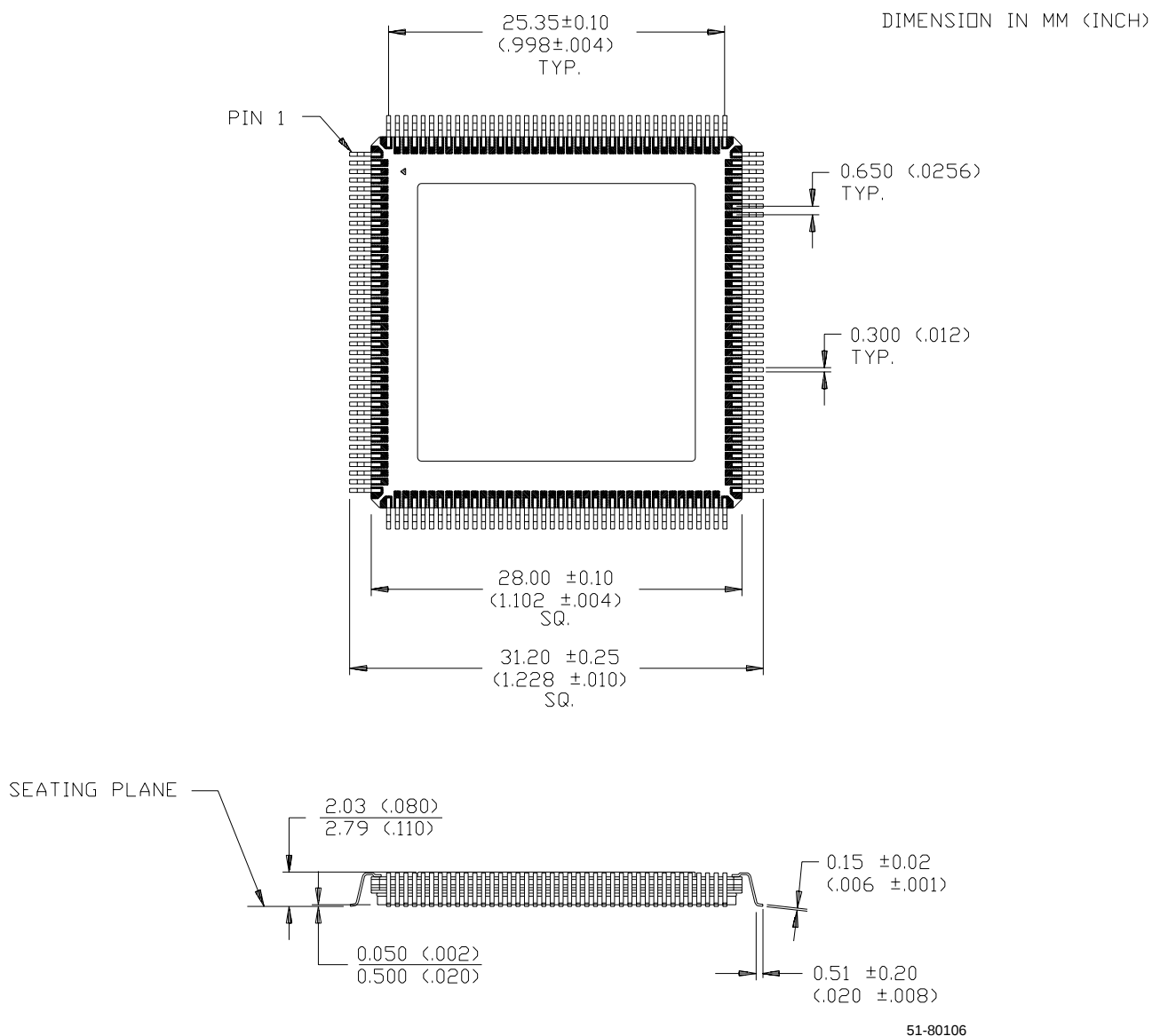
160-Lead Ceramic Quad Flatpack (Cavity Up) U162
