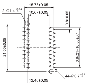
TSOP IC235-0442-207 (44 Pins)
