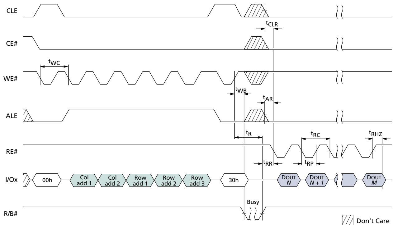
Figure 39: PAGE READ Operation
