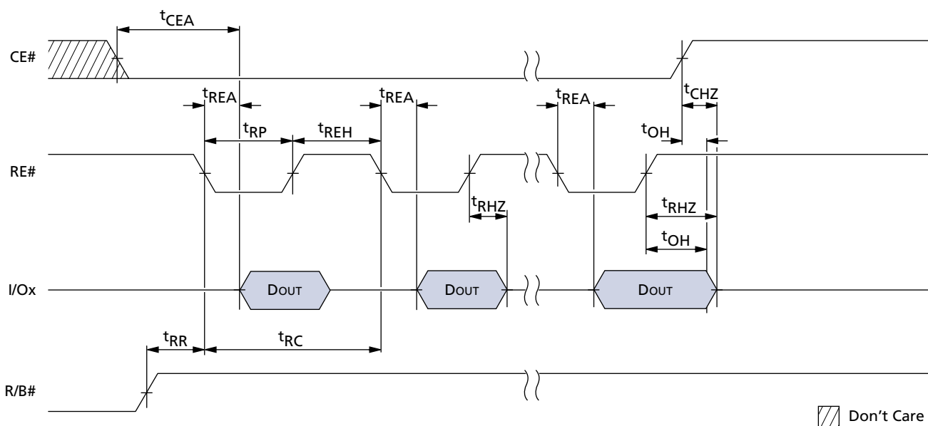
Figure 37: SERIAL ACCESS Cycle After READ
