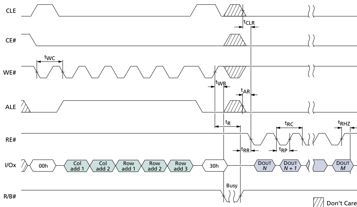
Figure 14: PAGE READ Operation
