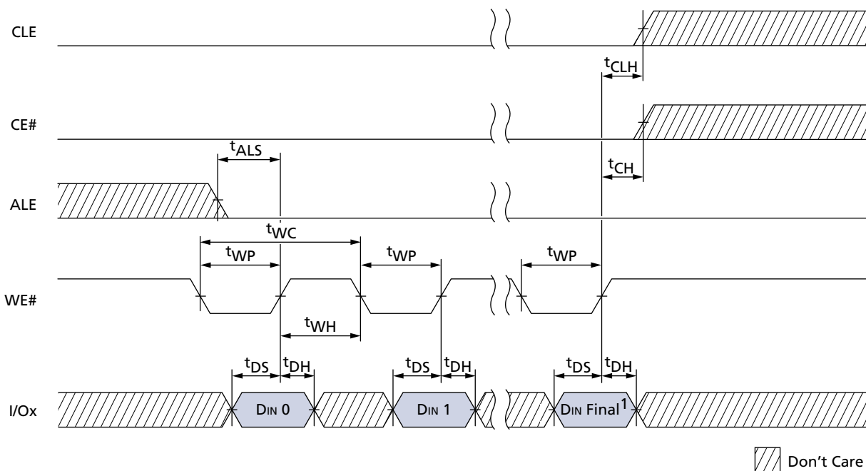
Figure 36: INPUT DATA LATCH Cycle
