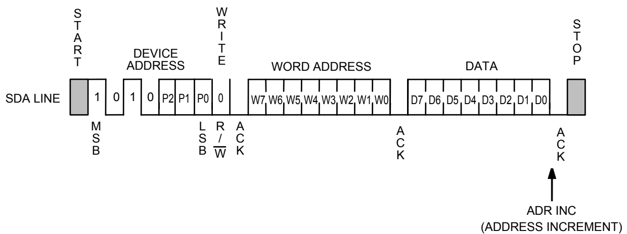
Figure 14 Byte Write
