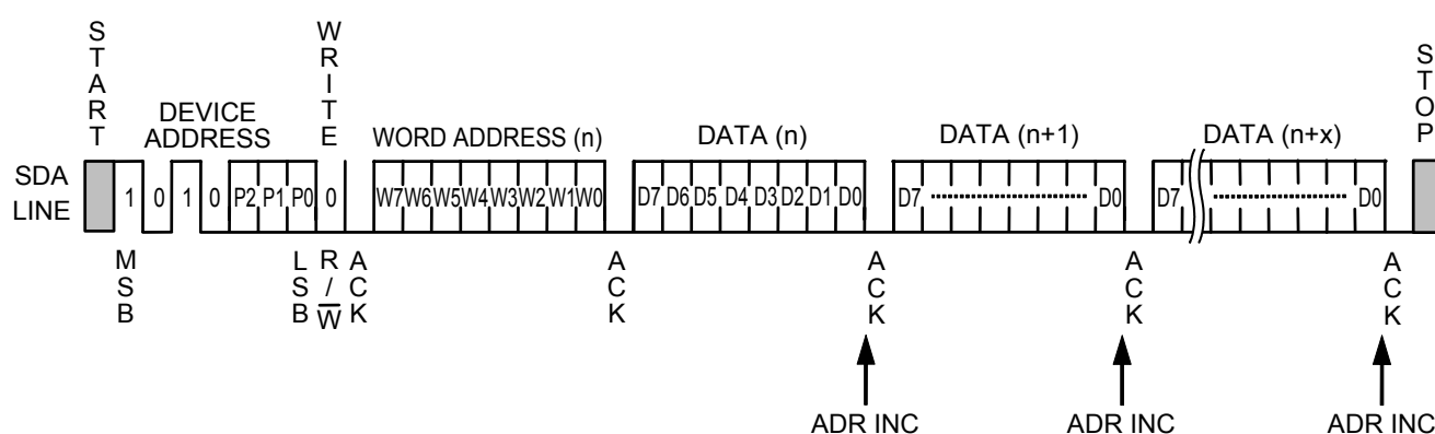
Figure 15 Page Write
