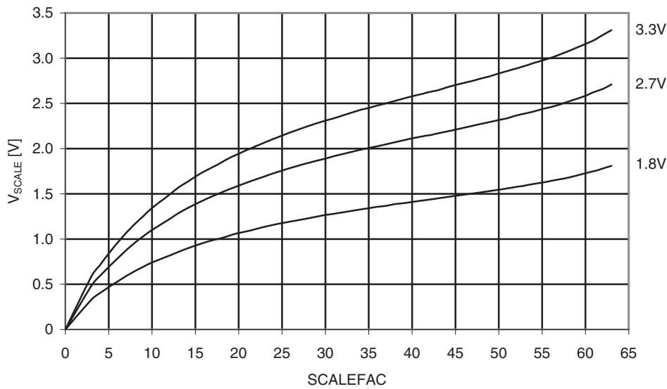
Figure 34-8. Analog comparator voltage scaler vs. scalefac.
