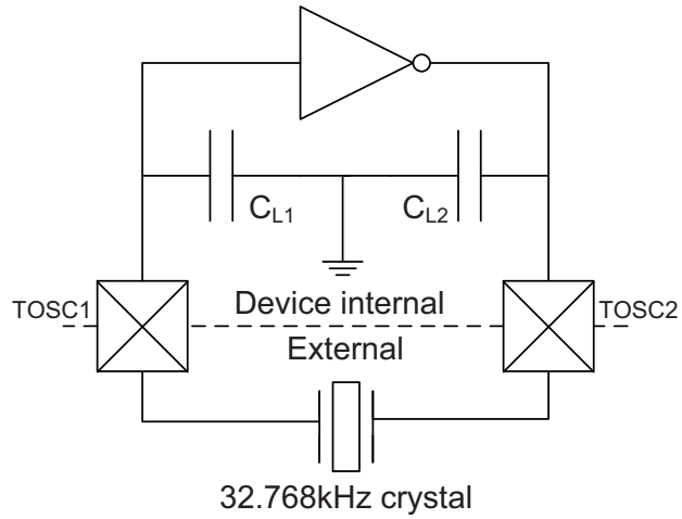
Figure 32-11. TOSC input capacitance.
