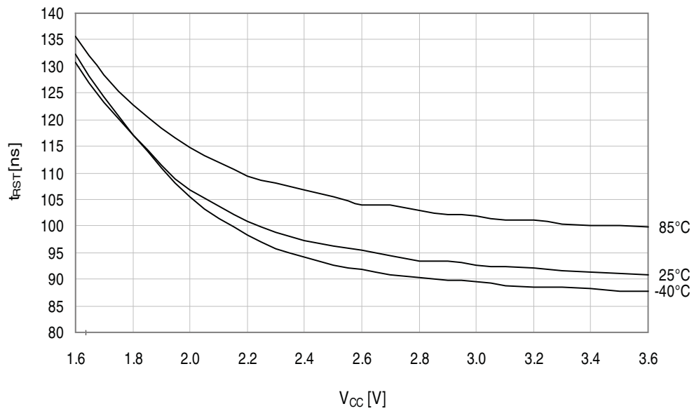
Figure 33-199. Minimum reset pin pulse width vs. V CC .
