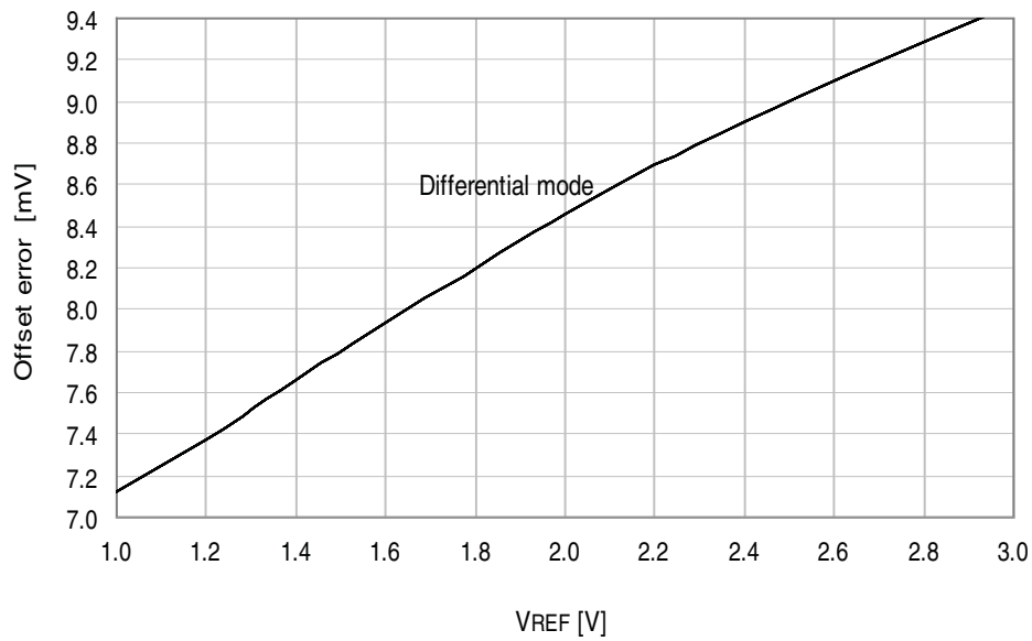
Figure 33-256. Offset error vs. V_{REF} . T = 25^{\circ}\text{C} , V_{CC} = 3.6\text{V} , \text{ADC sample rate} = 300\text{kpsps} .
