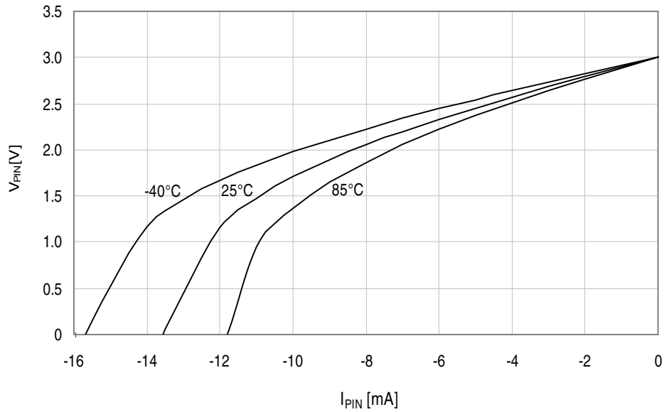
Figure 33-240. I/O pin output voltage vs. source current. V_{CC} = 3.0V .
