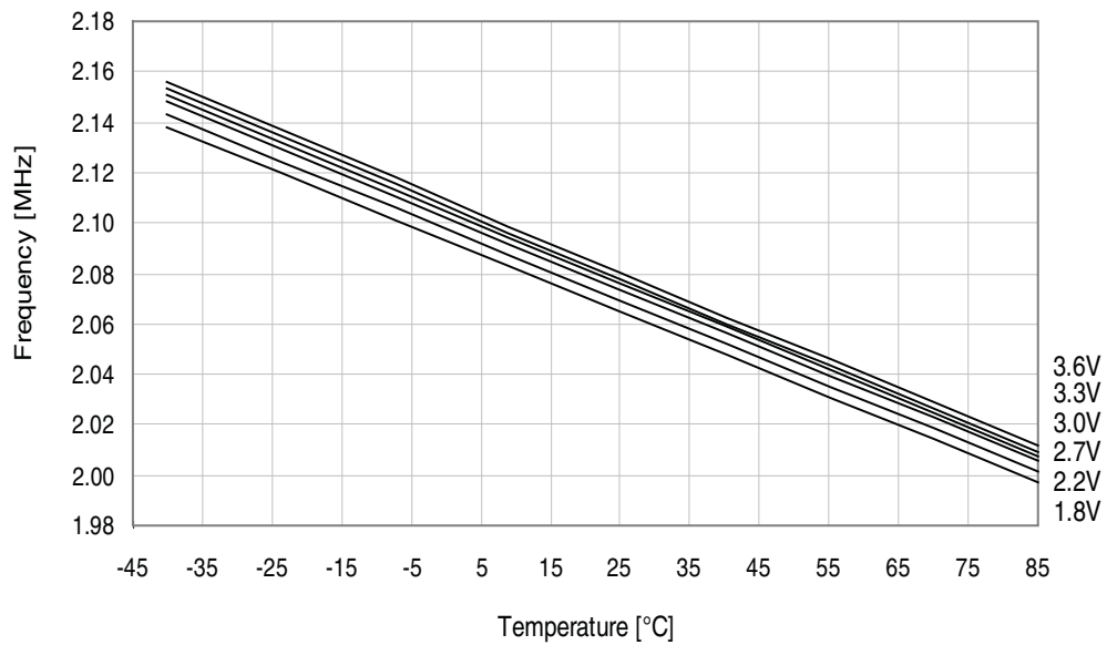
Figure 33-274. 2MHz internal oscillator frequency vs. temperature.
