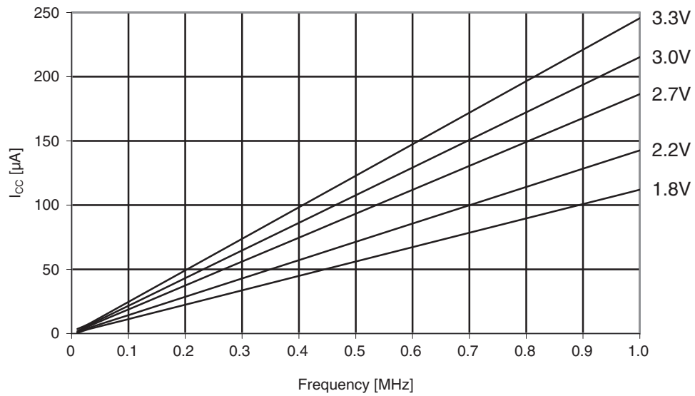
Figure 33-50. Idle supply current vs. frequency. f_{SYS} = 0 - 1.0MHz , T = 25°C .
