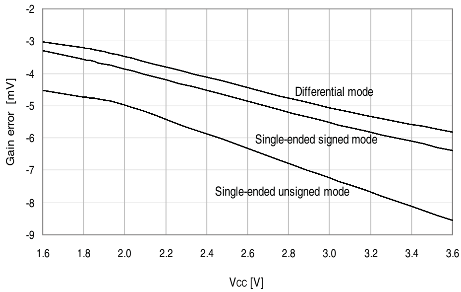
Figure 33-255. Gain error vs. V_{CC} . T = 25^{\circ}\text{C} , V_{REF} = \text{external } 1.0\text{V} , \text{ADC sample rate} = 300\text{kpsps} .
