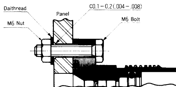
Mounting Method (2)
