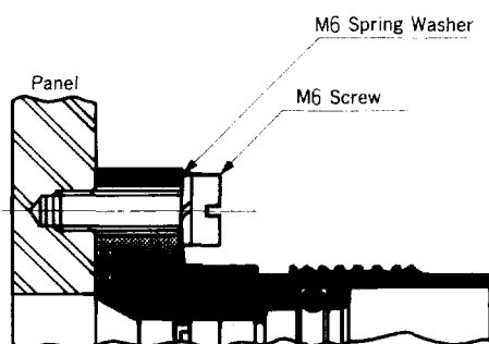
Mounting Method (1)
