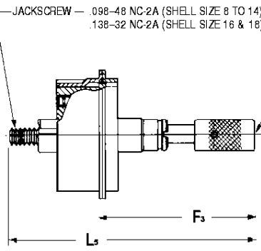
TYPE BA1 TYPE BA2
