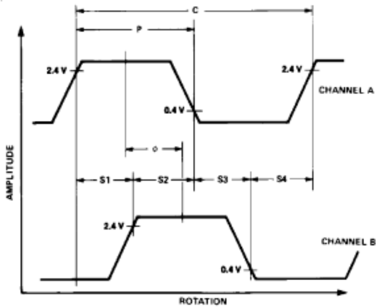
Figure 2. Output waveforms
