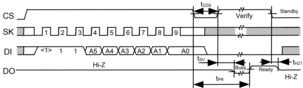
Figure 11 Data Erase Timing (S-93L46A)
