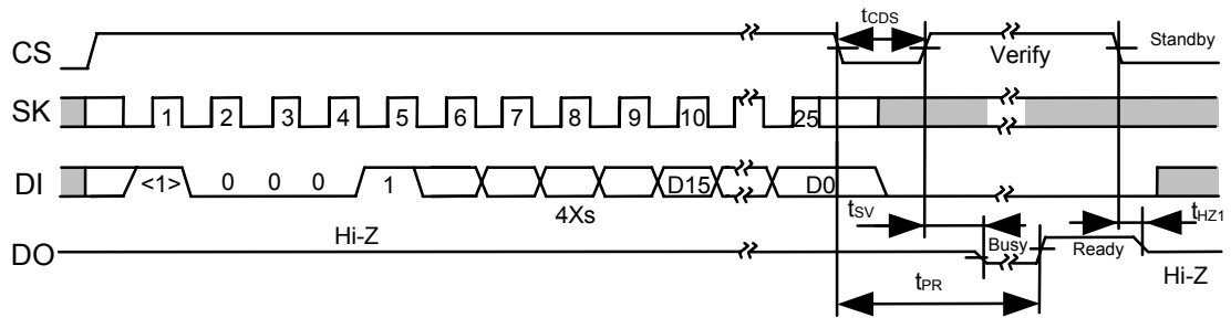
Figure 13 Chip Write Timing (S-93L46A)
