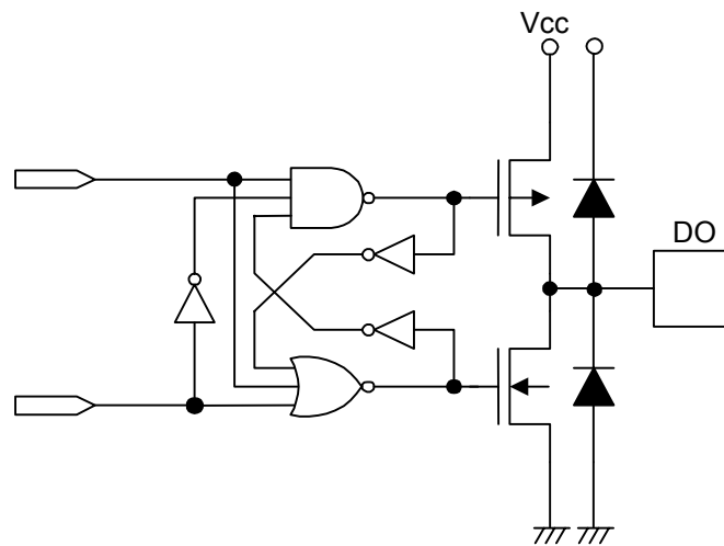
Figure 25 DO Pin
