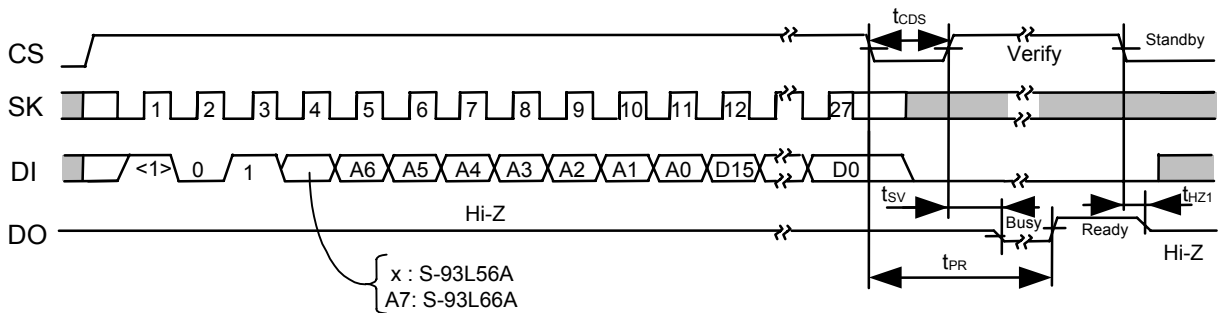
Figure 10 Data Write Timing (S-93L56A, S-93L66A)
