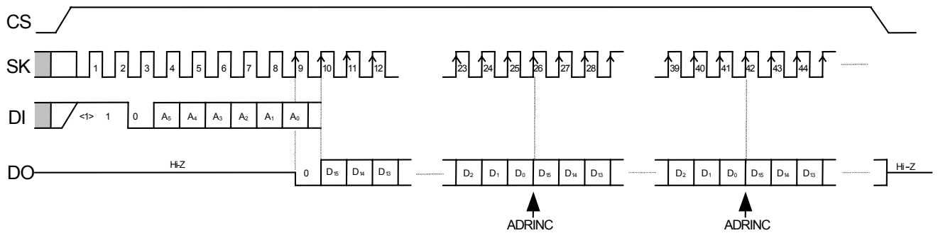
Figure 7 Read Timing (S-93L46A)
