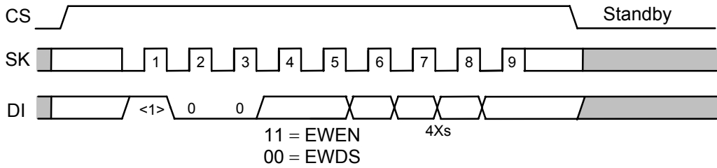
Figure 17 Write Enable/Disable Timing (S-93L46A)
