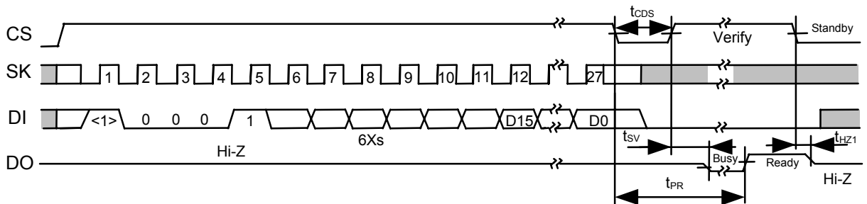
Figure 14 Chip Write Timing (S-93L56A, S-93L66A)
