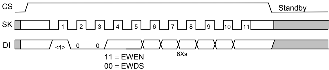
Figure 18 Write Enable/Disable Timing (S-93L56A, S-93L66A)
