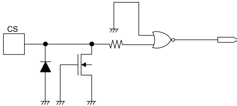
Figure 22 CS Pin
