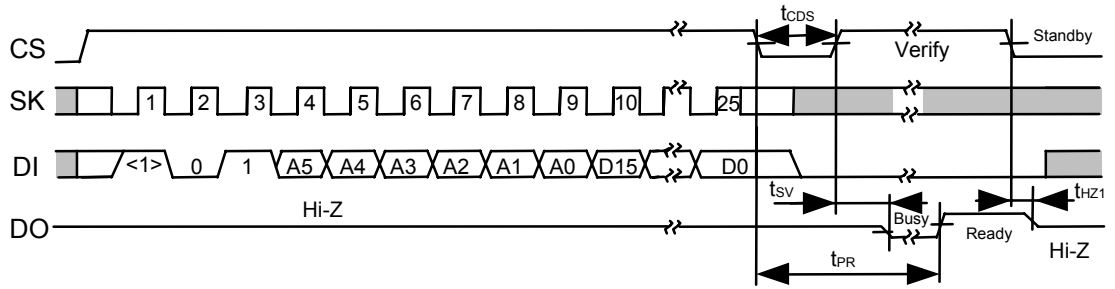
Figure 9 Data Write Timing (S-93L46A)
