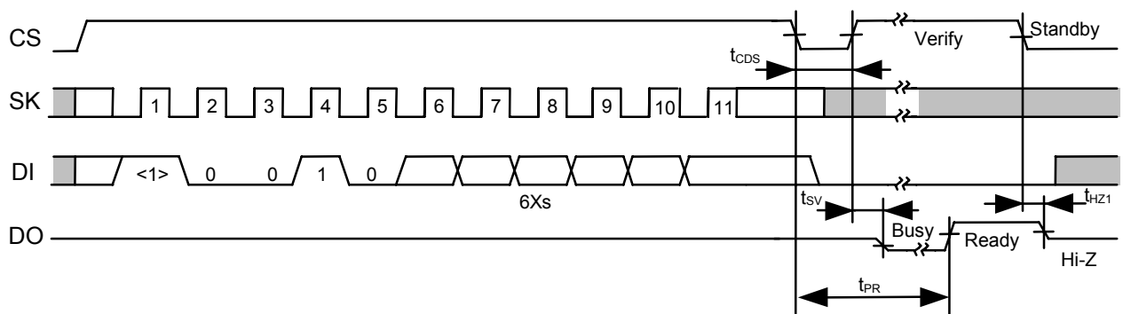
Figure 16 Chip Erase Timing (S-93L56A, S-93L66A)
