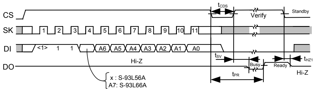
Figure 12 Data Erase Timing (S-93L56A, S-93L66A)
