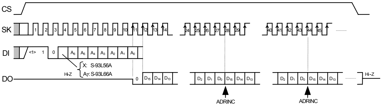
Figure 8 Read Timing (S-93L56A, S-93L66A)
