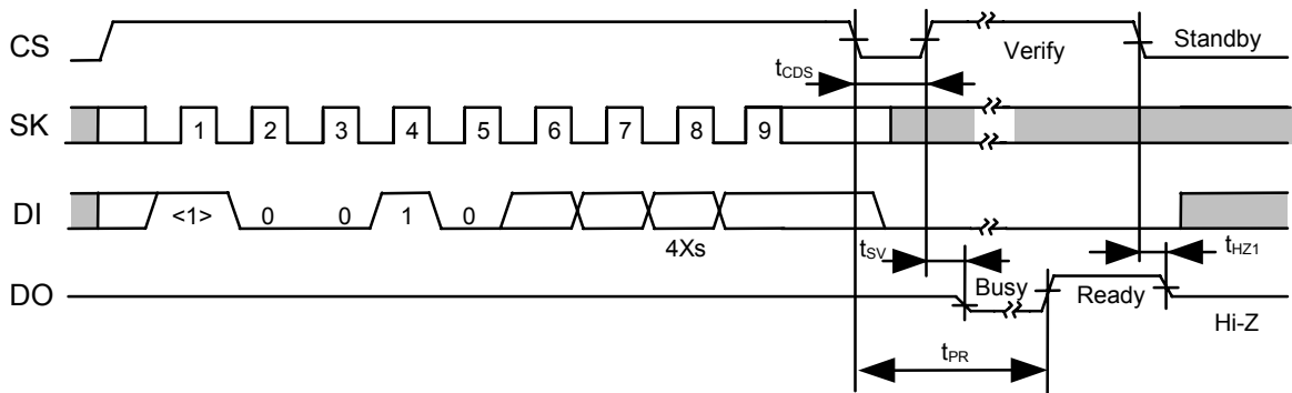
Figure 15 Chip Erase Timing (S-93L46A)
