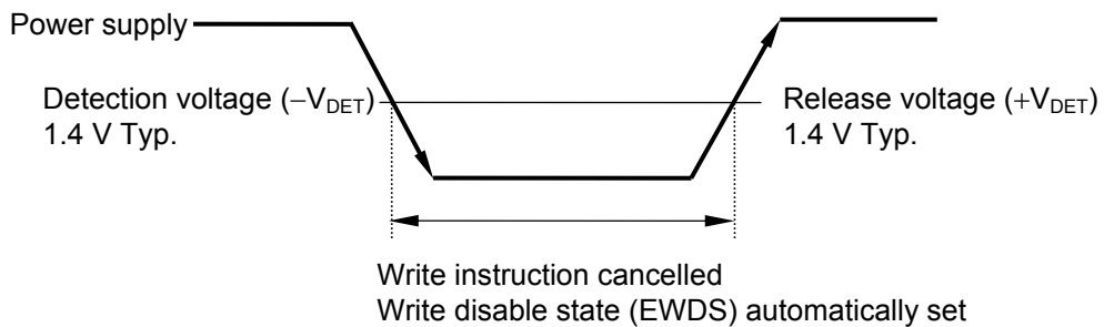
Figure 19 Operation when Power Supply Voltage is Low
