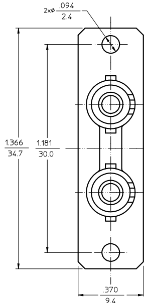
RECOMMENDED MOUNTING PATTERN
