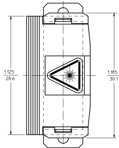
VIEW A VARIATION 2 FOR LABEL INSTALLATION
