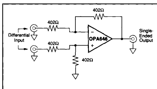
FIGURE 13. Unity Gain Difference Amplifier.
