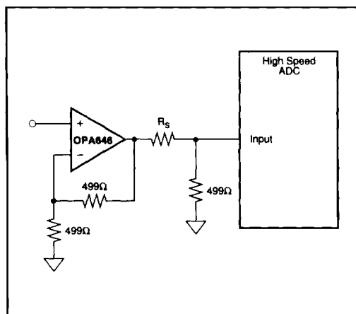
FIGURE 14. Differential Input Buffer Amplifier ( G = +2V/V ).
