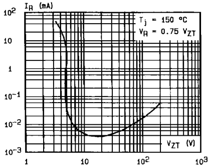
Fig.6 - Reverse current versus regulation voltage (typical values).
