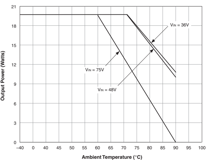
Temperature Derating Curves for UEP-3.3/6000-D48
