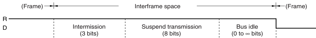
Figure 19-14. Interframe Space (Error Passive Node)
