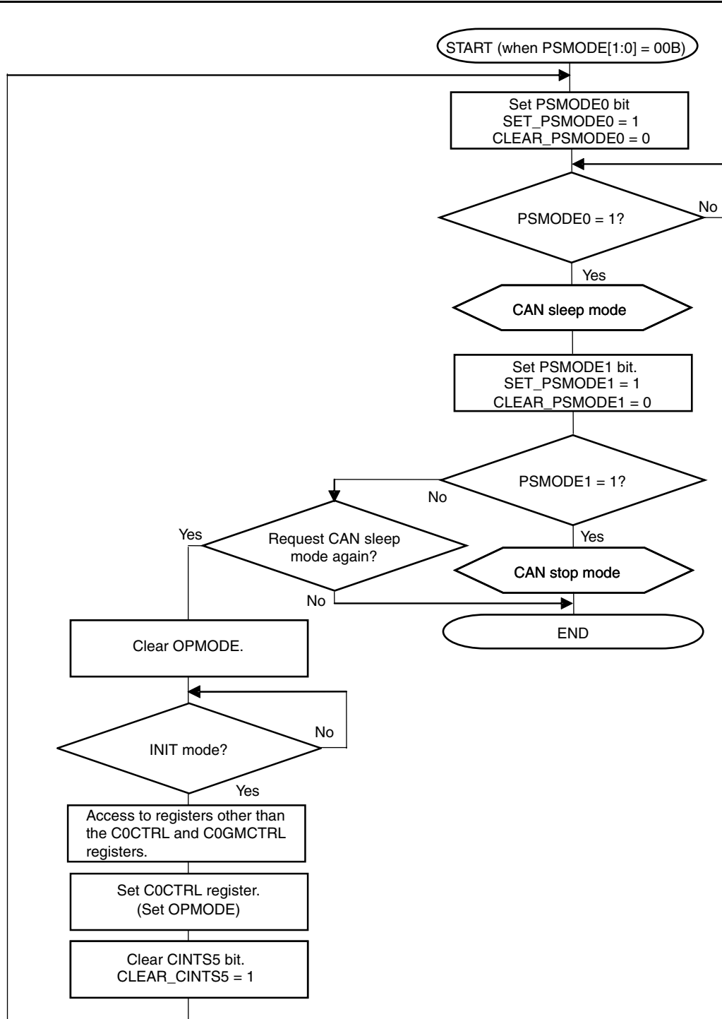
Figure 19-52. Setting CAN Sleep Mode/Stop Mode
