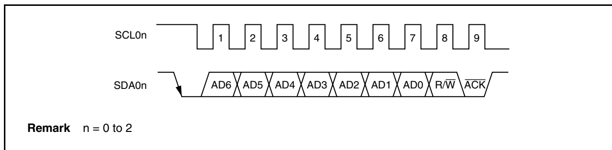
Figure 17-11. \overline{\text{ACK}}
