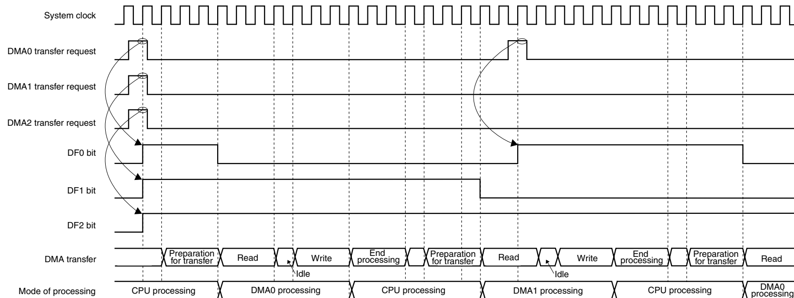
Figure 20-2. Priority of DMA (2)
