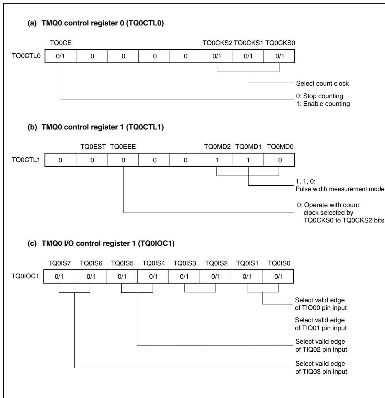
Figure 8-40. Register Setting in Pulse Width Measurement Mode (1/2)
