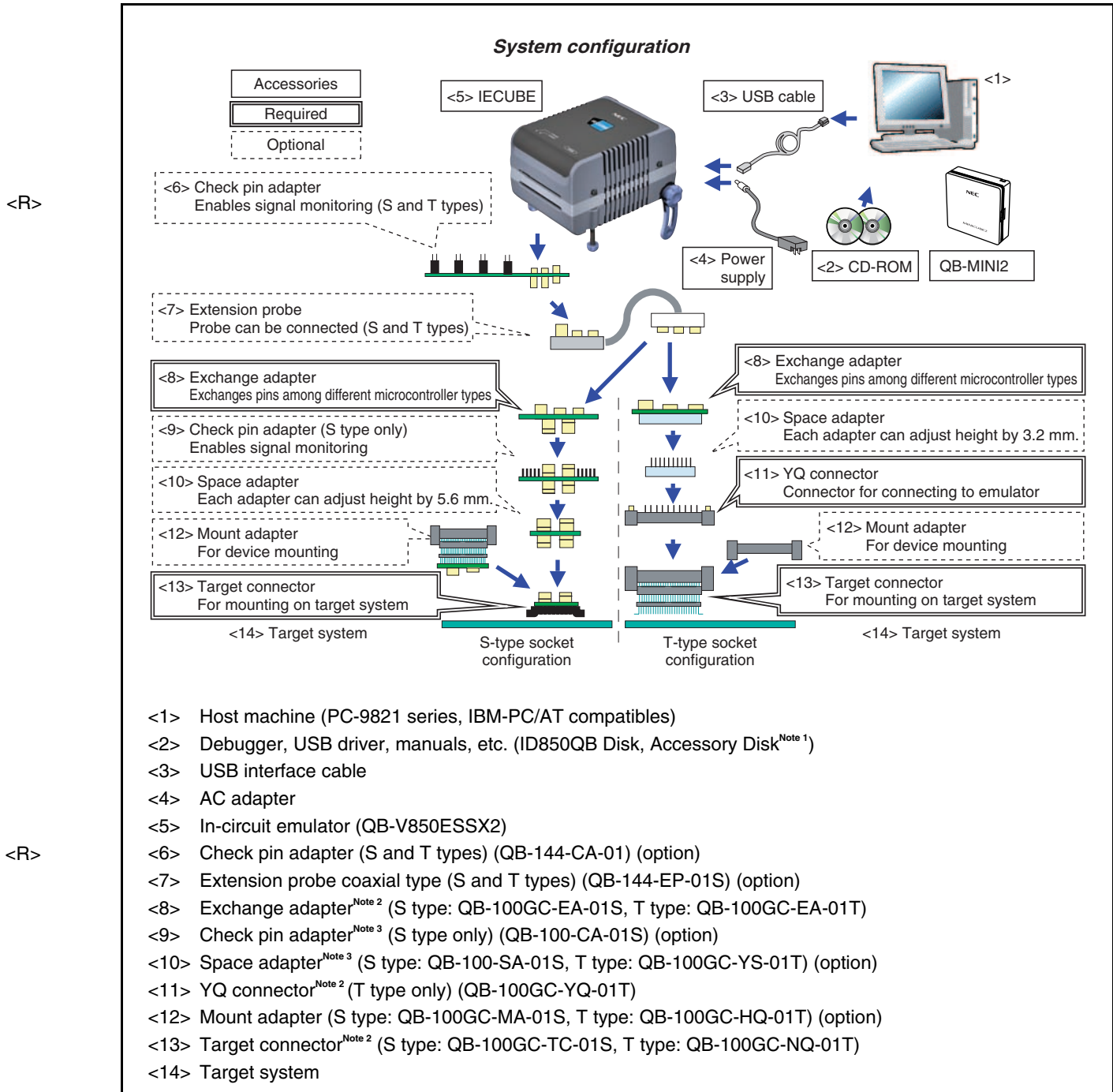
Figure A-3. System Configuration (QB-V850ESSX2 Used) (1/2)
