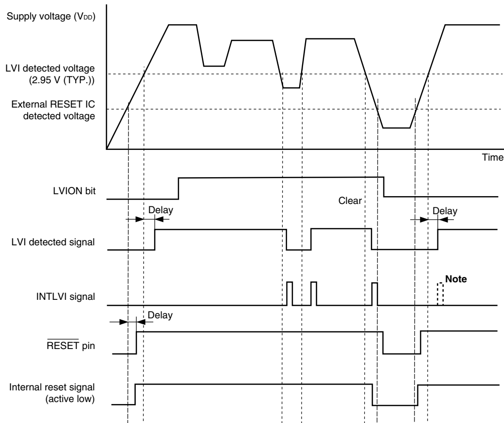
Figure 27-3. Operation Timing of Low-Voltage Detector (LVIMD Bit = 0)
