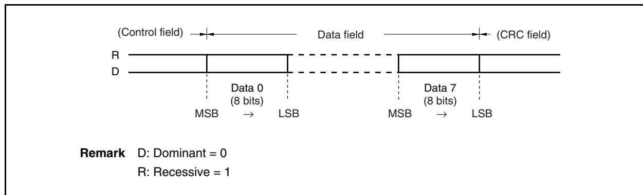
Figure 19-9. Data Field
