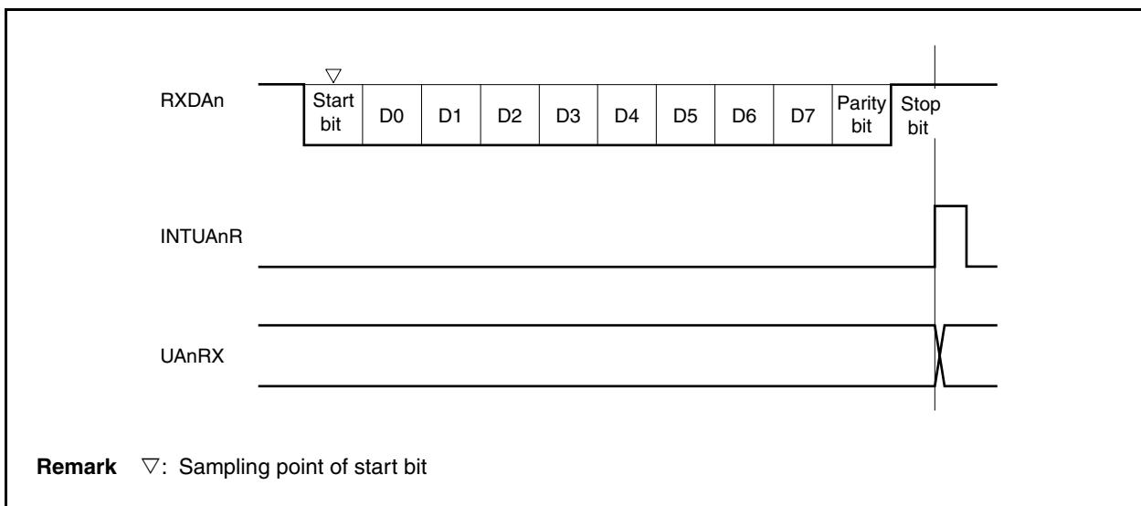
Figure 15-13. UART Reception
