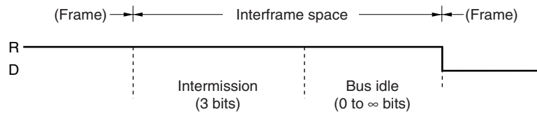
Figure 19-13. Interframe Space (Error Active Node)
