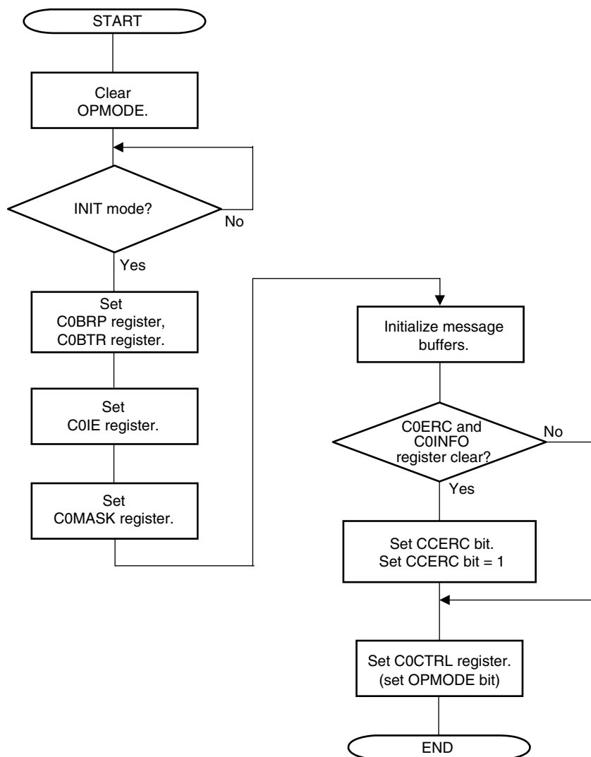
Figure 19-37. Re-initialization
