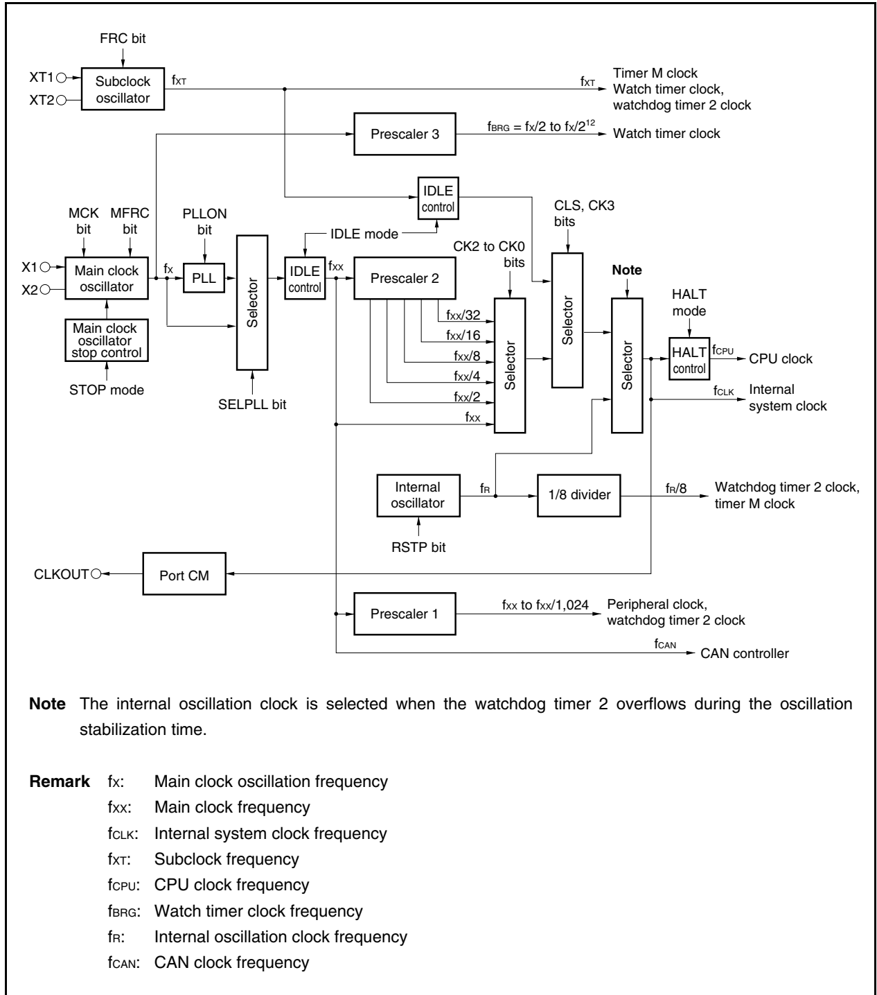
Figure 6-1. Clock Generator
