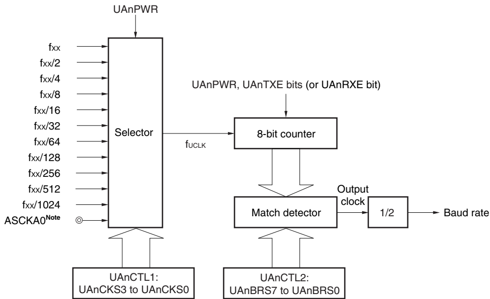
Figure 15-16. Configuration of Baud Rate Generator
