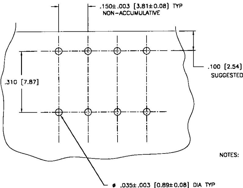
RECOMMENDED MOUNTING HOLE PATTERN SCALE 4/1
