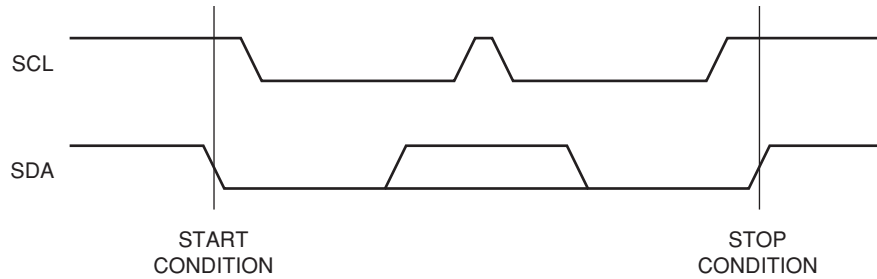
Figure 1. START/STOP Conditions
