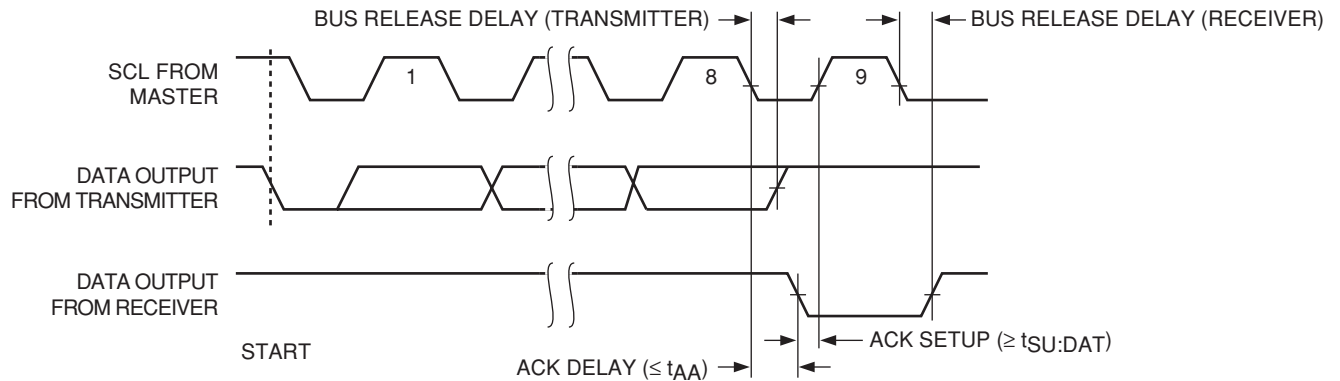
Figure 3. Acknowledge Timing
