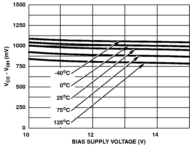
FIGURE 23. HIGH LEVEL OUTPUT VOLTAGE V_{CC} - V_{OH} vs BIAS SUPPLY VOLTAGE AND TEMPERATURE AT 100mA
