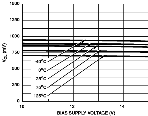
FIGURE 24. LOW LEVEL OUTPUT VOLTAGE V_{OL} vs BIAS SUPPLY VOLTAGE AND TEMPERATURE AT 100mA
