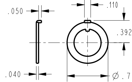
LOCKING RING 3
