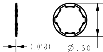
LOCKWASHER 3
