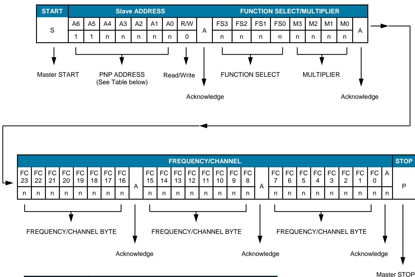
Figure 2: I 2 C Bus Data Structure
