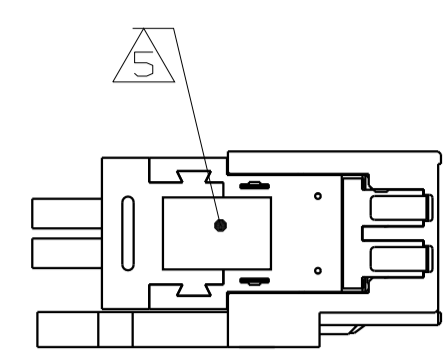
RECEPTACLE, PUSH TO RELEASE 2 PAIR X 10 NATURAL
