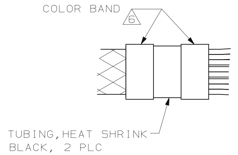
COLOR BAND DETAIL -10 THRU -16
