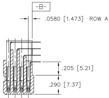
SECTION X-X
