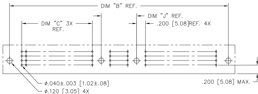
SECTION U-U
