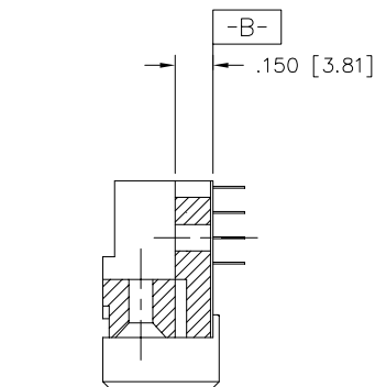
SECTION W-W
