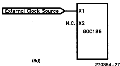
Figure 8. 80C186 Oscillator Configurations (see text)
