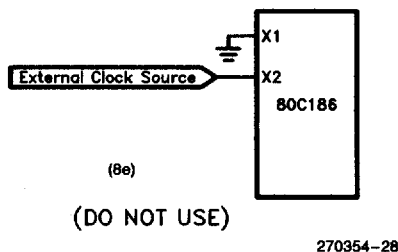
Figure 8. 80C186 Oscillator Configurations (see text)
