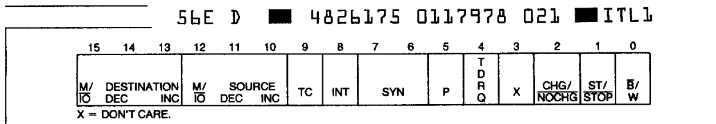
Figure 17. DMA Control Register
