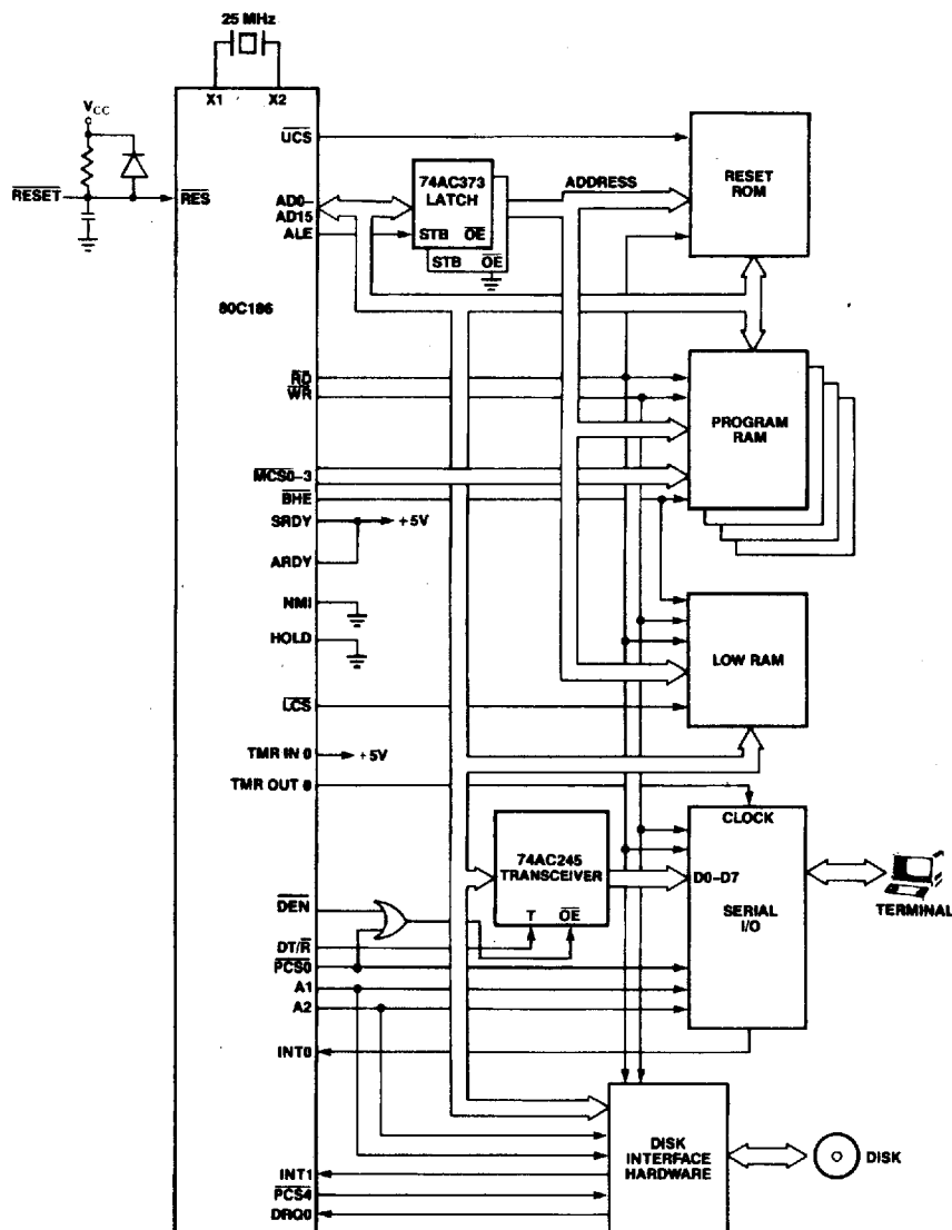
Figure 45. Typical 80C186 Computer
