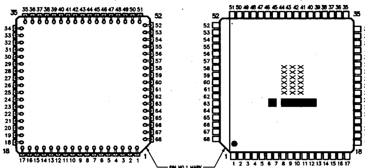
Figure 2. 80C186 Pinout Diagrams
