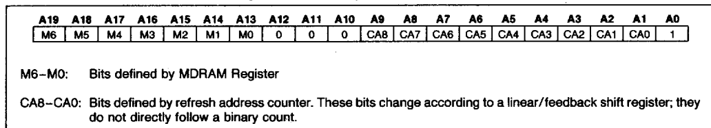
Figure 41. Addresses Generated by RCU
