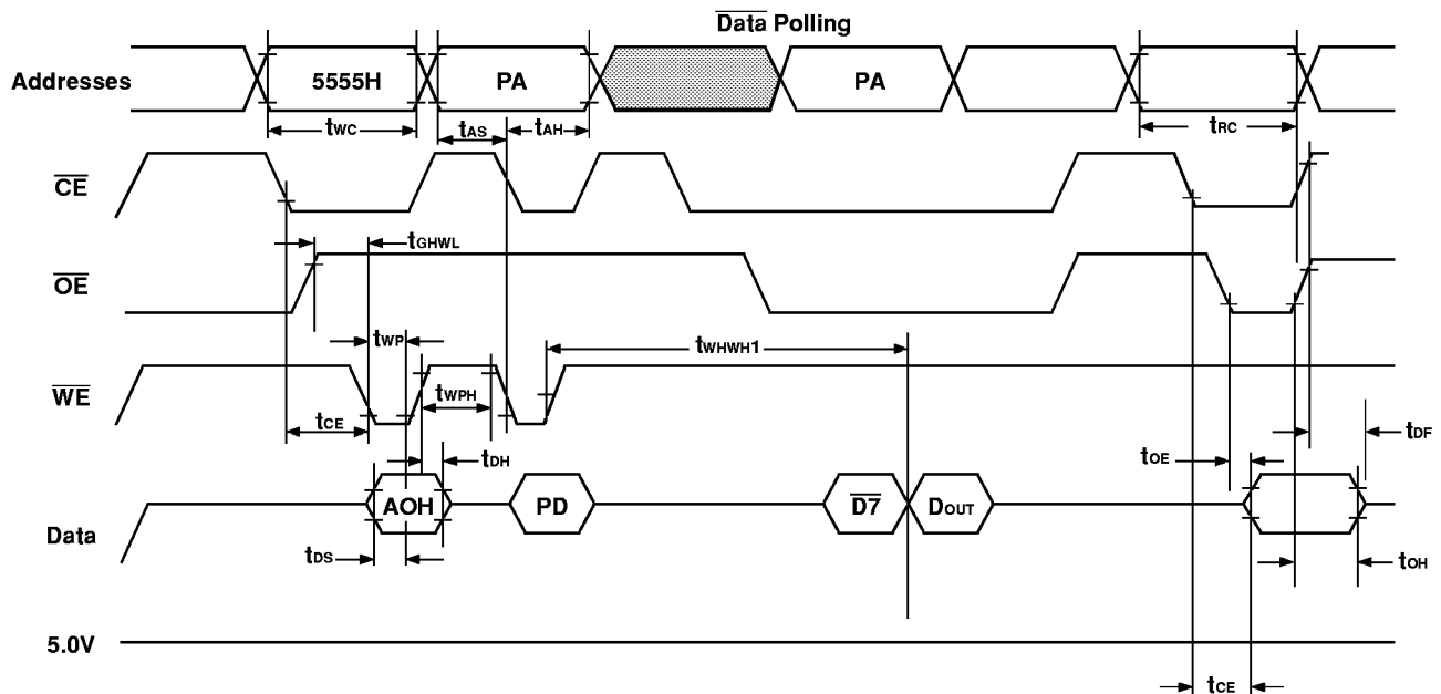
Figure 8 Write/Erase/Program Operation, \overline{WE} Controlled
