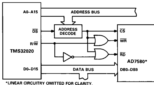
Figure 25. TMS32020 to AD7580 Interface
