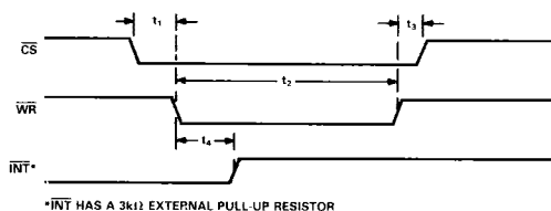
Figure 1. AD7579/AD7580 Start Cycle Timing
