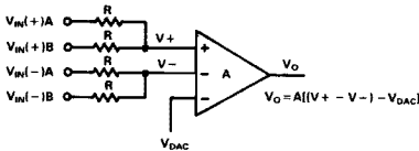
Figure 6. AD7579/AD7580 Input Circuit
