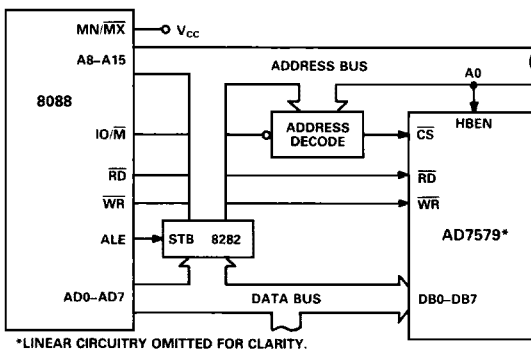
Figure 24. 8088 to AD7579 Interface
