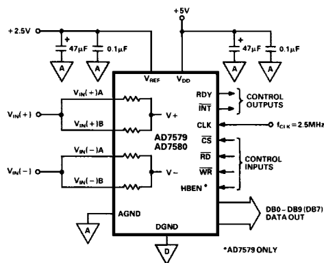
Figure 12. Unipolar 2.5V Operational Diagram
