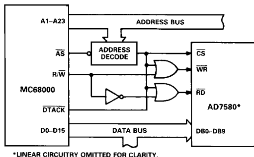
Figure 23. MC68000 to AD7580 Interface
