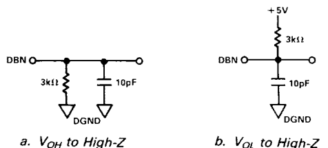
Figure 4. Load Circuits for Output Float Delay ( t_{13} )
