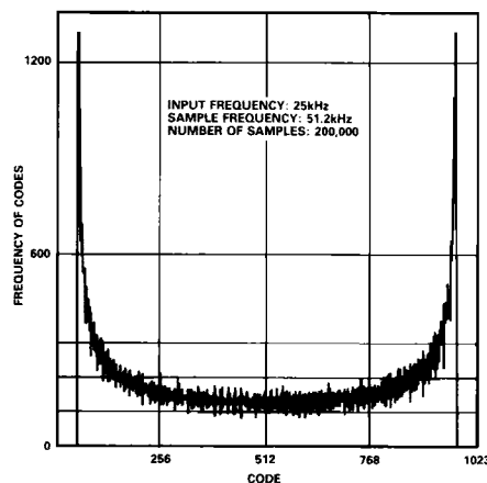
Figure 22. Histogram Plot for AD7579/AD7580
