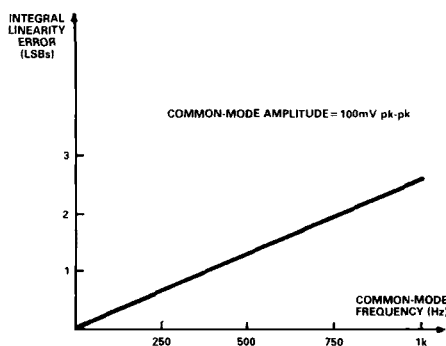
Figure 9. AD7579/AD7580 Error vs. Common-Mode Frequency
