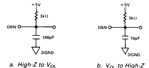
Figure 5. Load Circuit for \overline{INT} Propagation Delays
