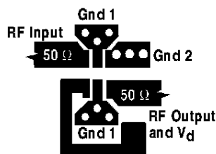
Figure 11. RF Layout.
