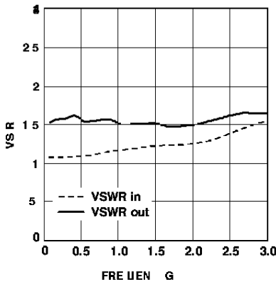
Figure 7. Input and Output VSWR vs. Frequency.
