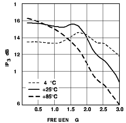
Figure 9. Third Order Intercept Point, IP_3 vs. Frequency and Temperature.
