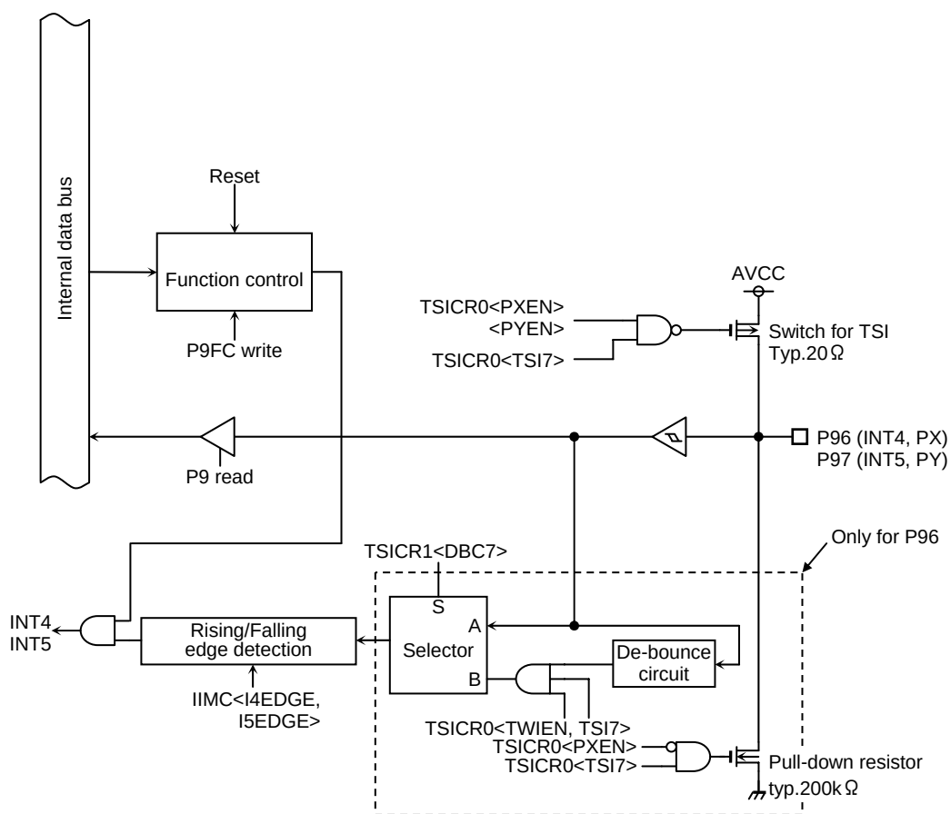
Figure 3.5.16 Port 96, 97
