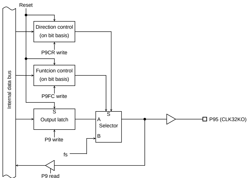
Figure 3.5.15 Port 95
