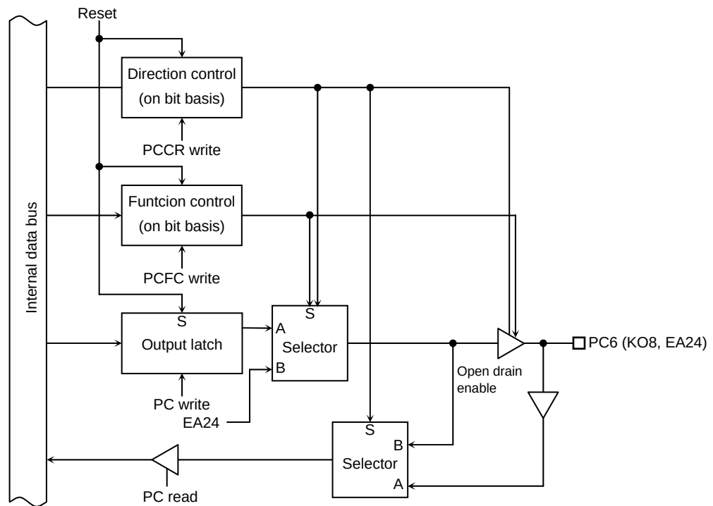
Figure 3.5.23 Port C6
