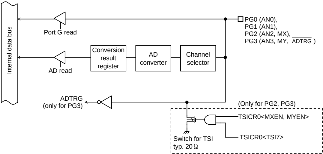
Figure 3.5.32 Port G
