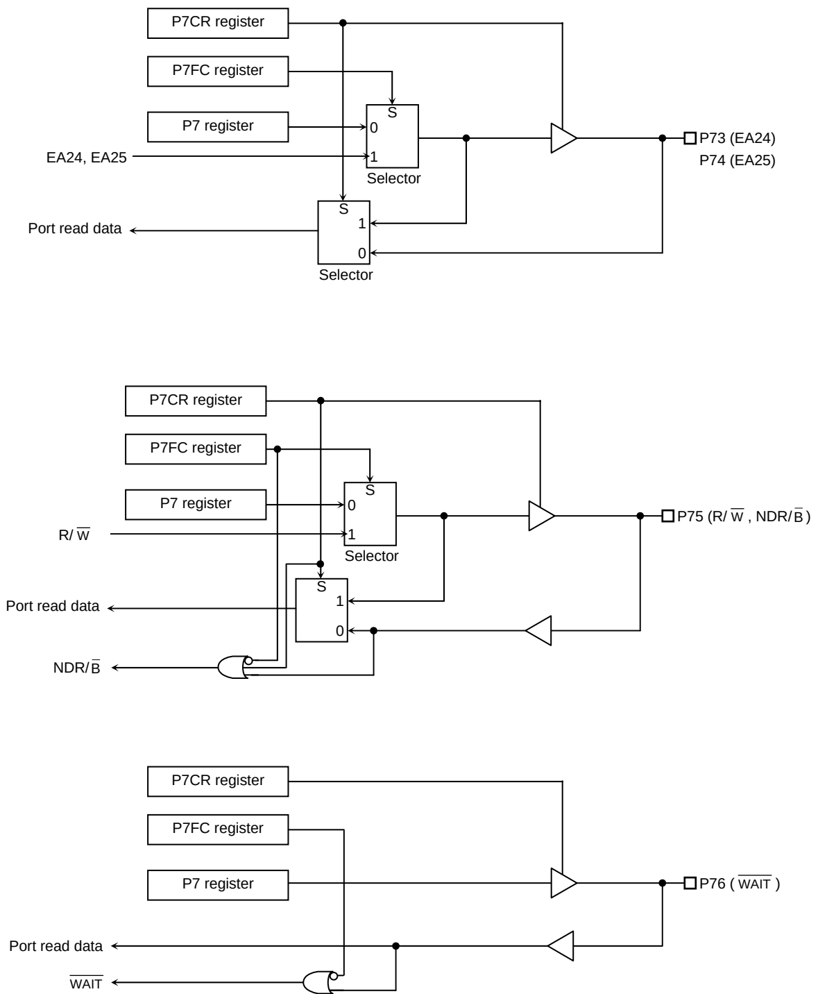
Figure 3.5.8 Port 7
