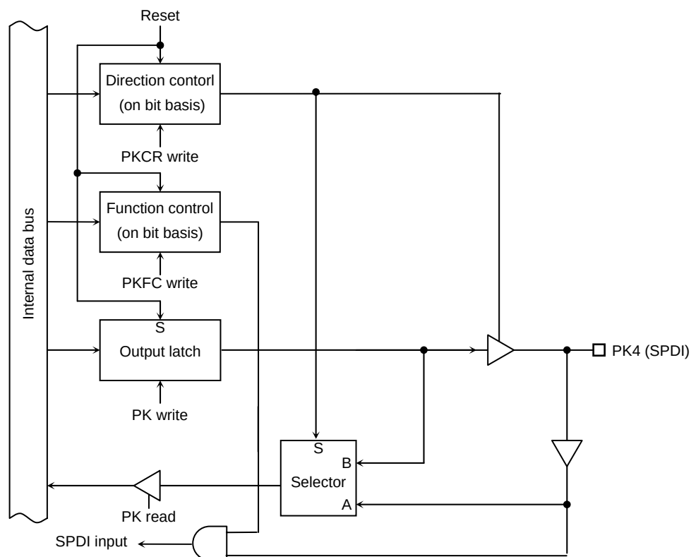
Figure 3.5.38 Port K4
