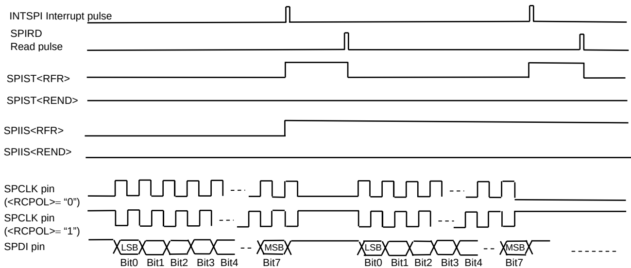
Figure 3.11.27 Micro DMA transmission (UNIT receiving (SPICT<RFUEN>=1))
