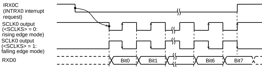
Figure 3.9.15 Receiving Operation in I/O Interface Mode (SCLK0 output mode)
