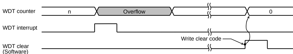
Figure 3.13.2 Normal Mode
