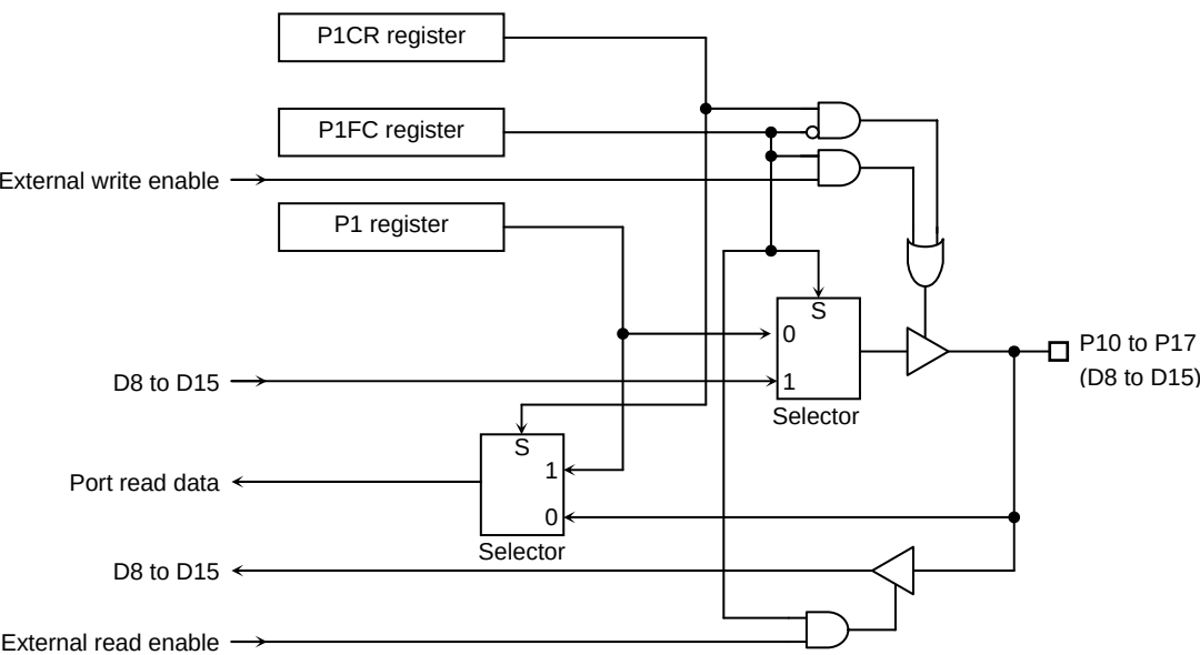
Figure 3.5.1 Port 1
