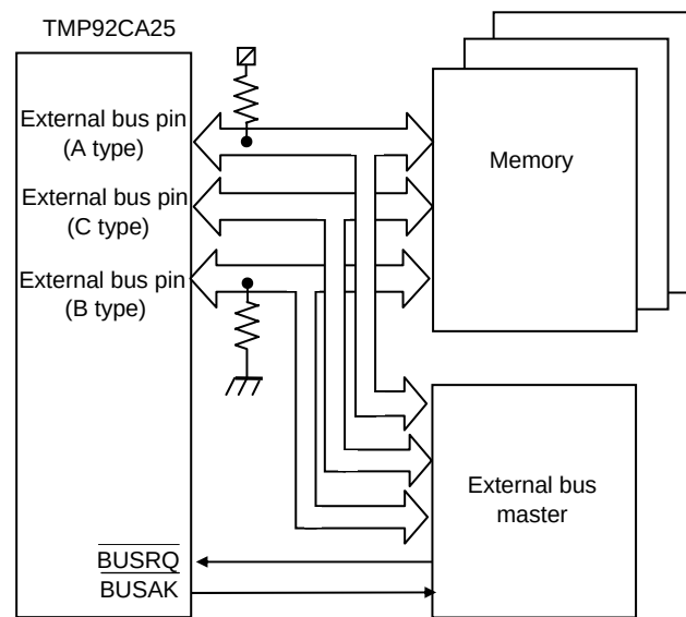
Figure 3.23.2 Connection example
