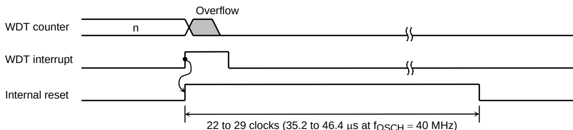
Figure 3.13.3 Reset Mode
