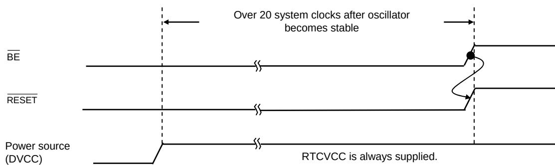
Figure 3.22.4 Shift from PSB Mode to NORMAL Mode
