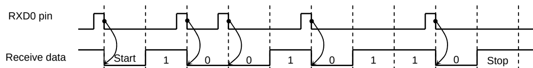
Figure 3.9.20 Receiving Example
