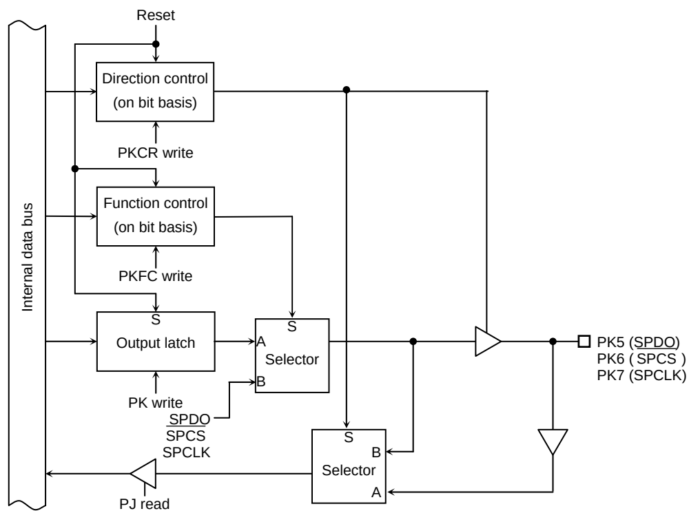
Figure 3.5.39 Port K5 to K7
