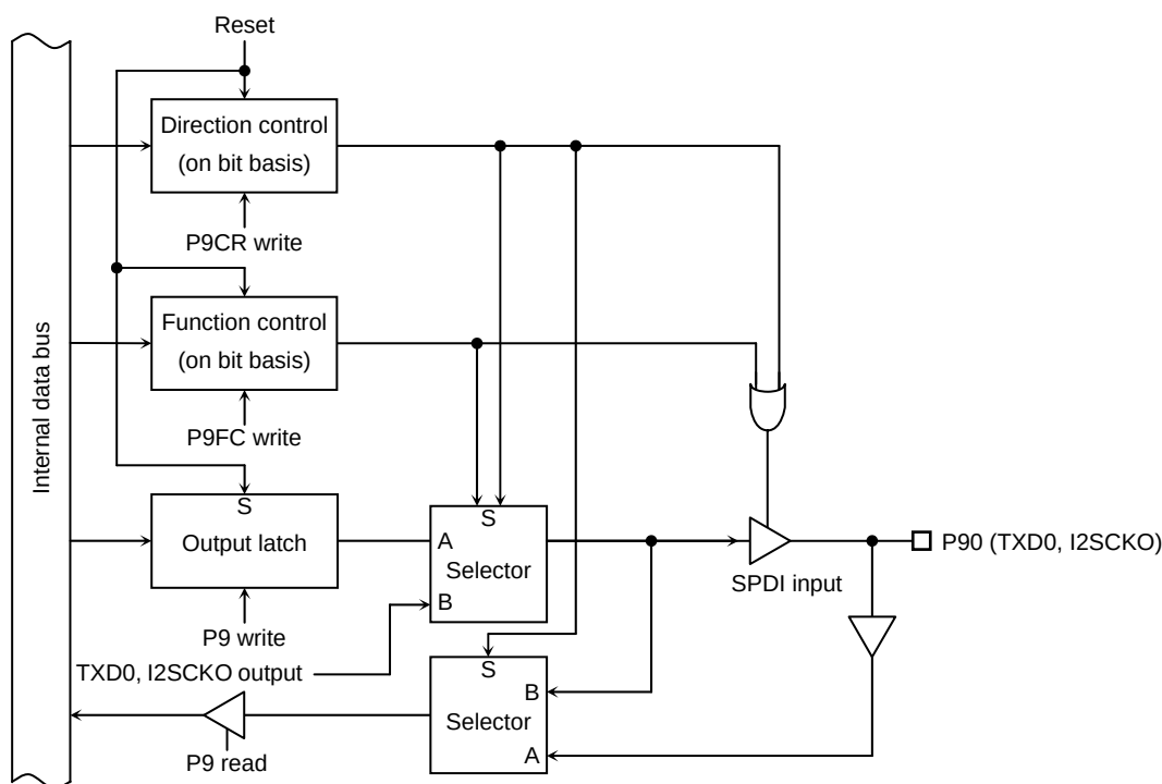
Figure 3.5.12 P90
