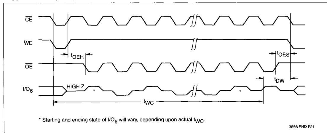
Toggle Bit Timing Diagram
