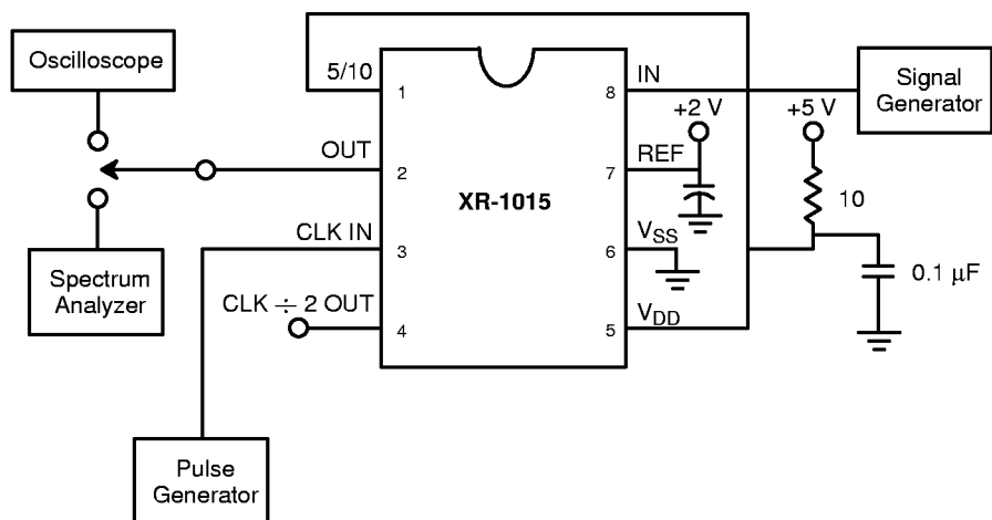
Figure 2. XR-1015 Test Circuit: 5 V Operation ( V_{DD} = +5 V, V_{SS} = 0 V, Ref = +2 V)
