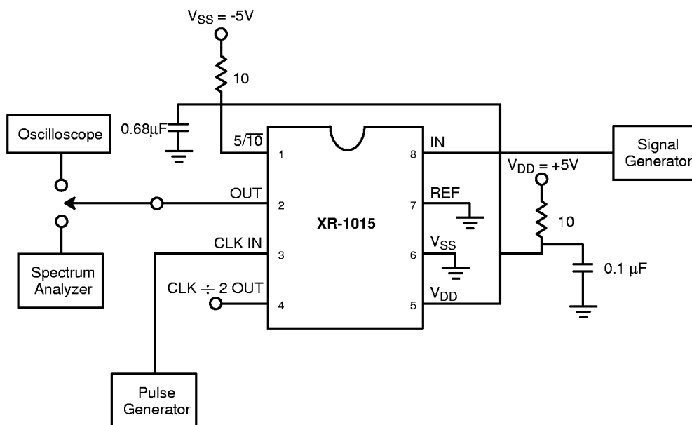
Figure 3. XR-1015 Test Circuit: 10 V Operation ( V_{DD} = +5 V, V_{SS} = -5 V)
